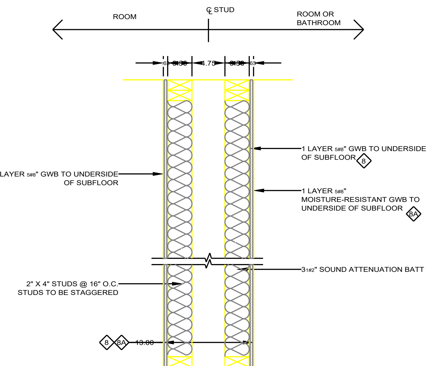
8 NON-RATED PLUMBING CHASE
