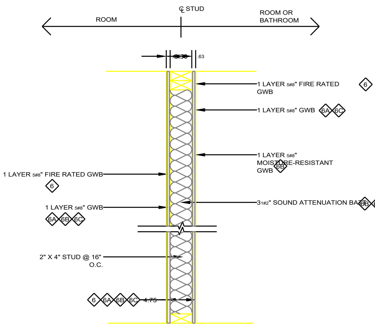
6 ONE HR RATED INTERIOR BEARING PARTITION
