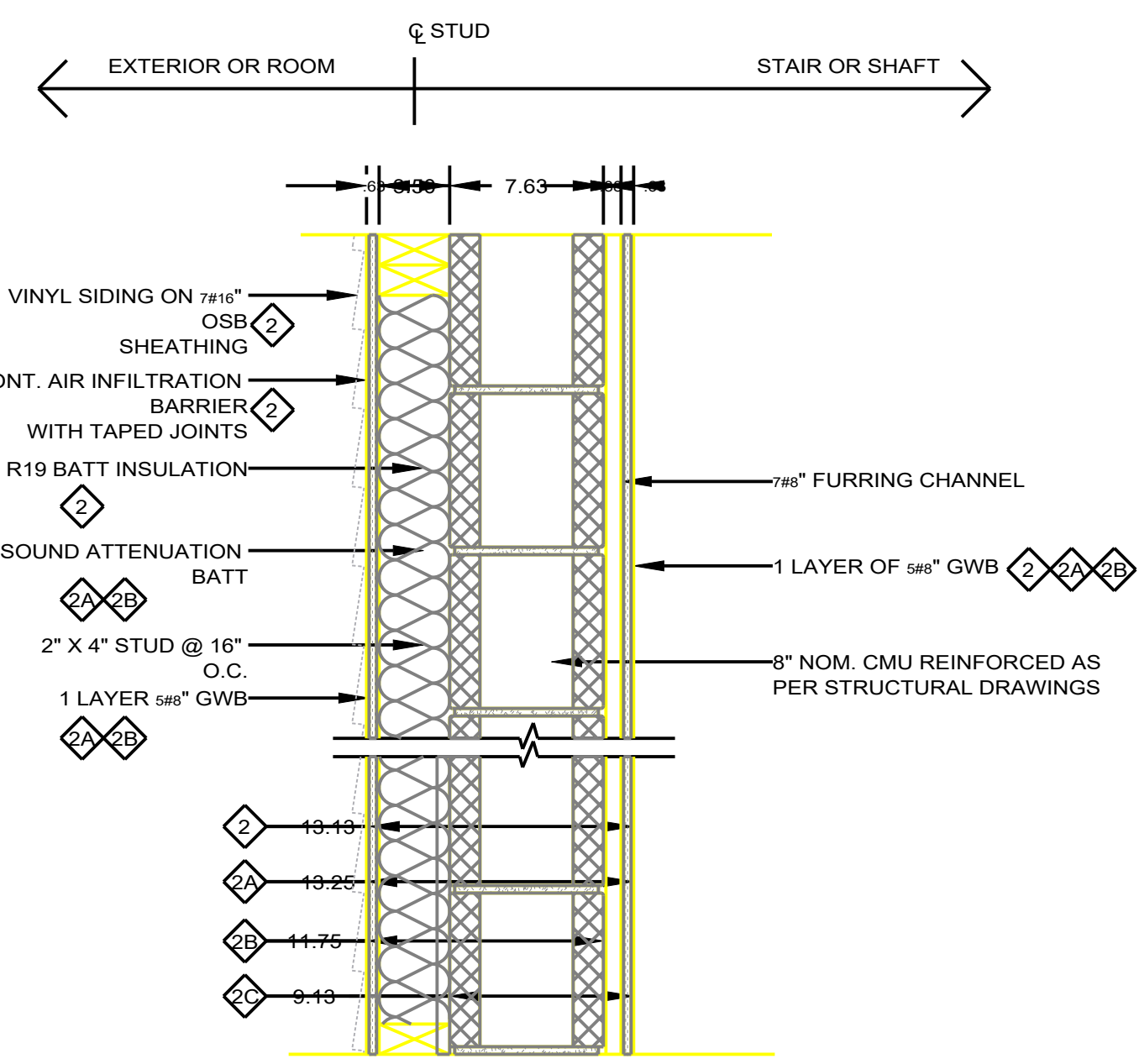
2 ONE HOUR RATED EXTERIOR MASONRY PARTITION
