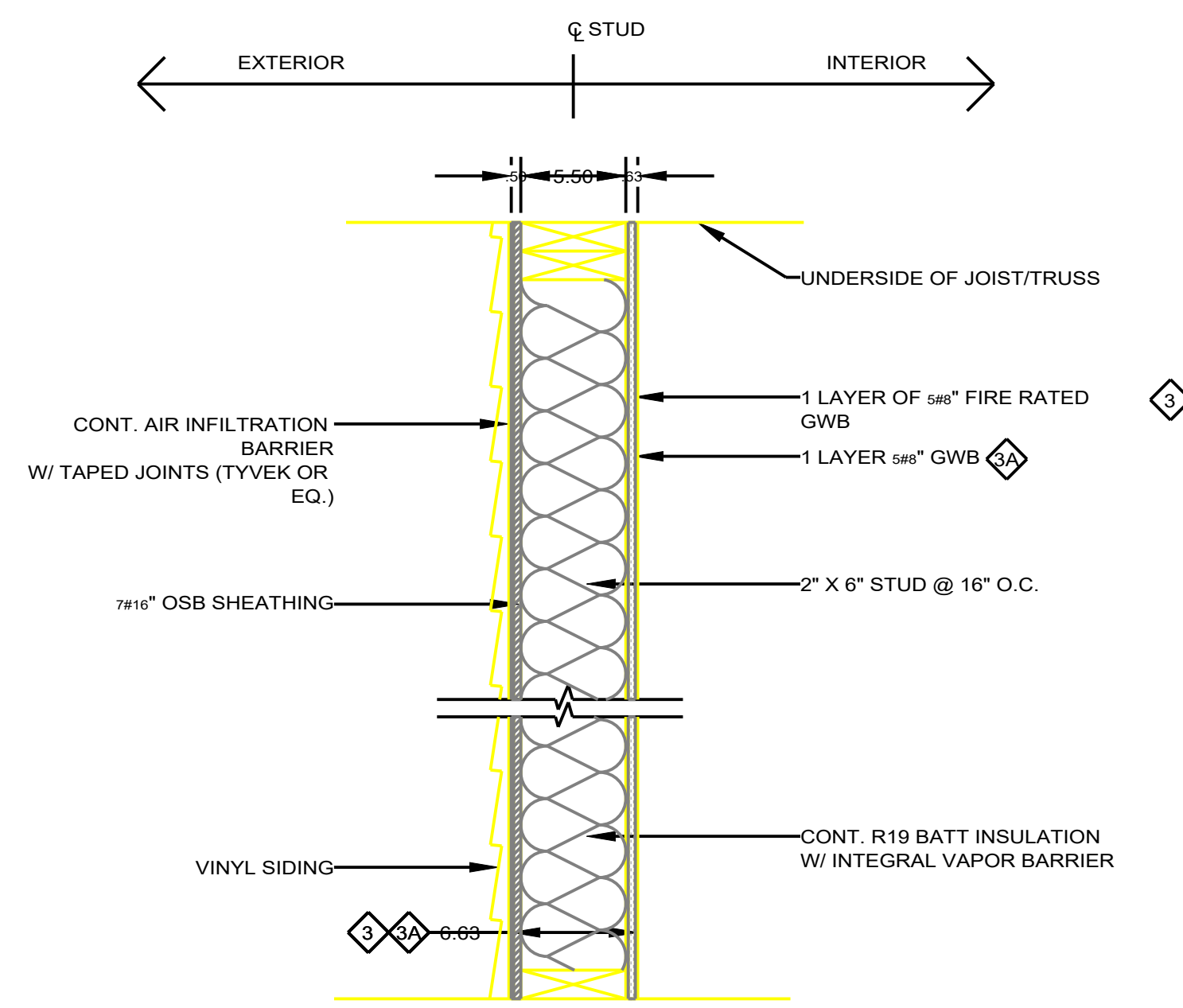
3 ONE HOUR RATED EXTERIOR BEARING PARTITION
