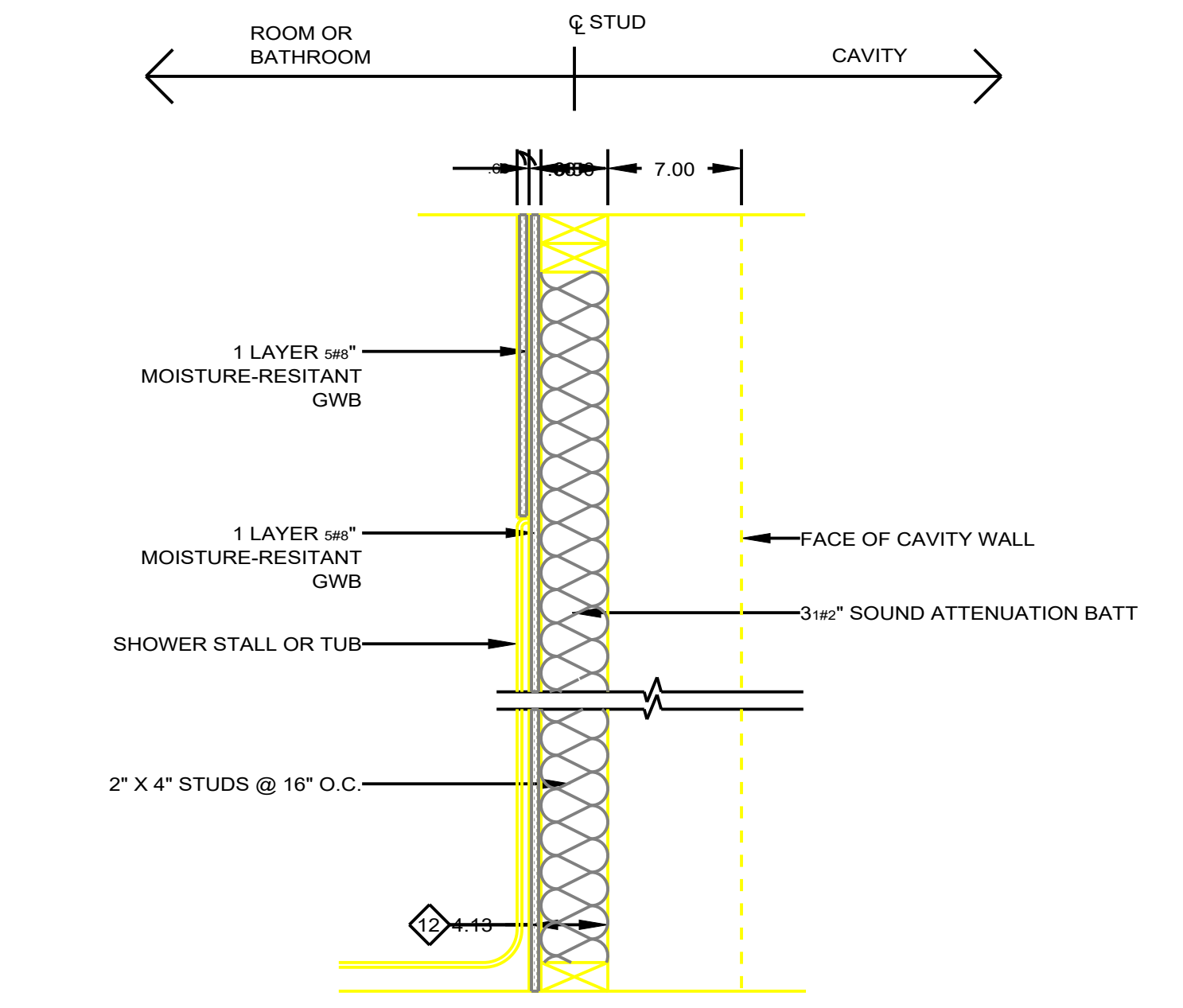
12 NON-RATED INTERIOR FURRING
