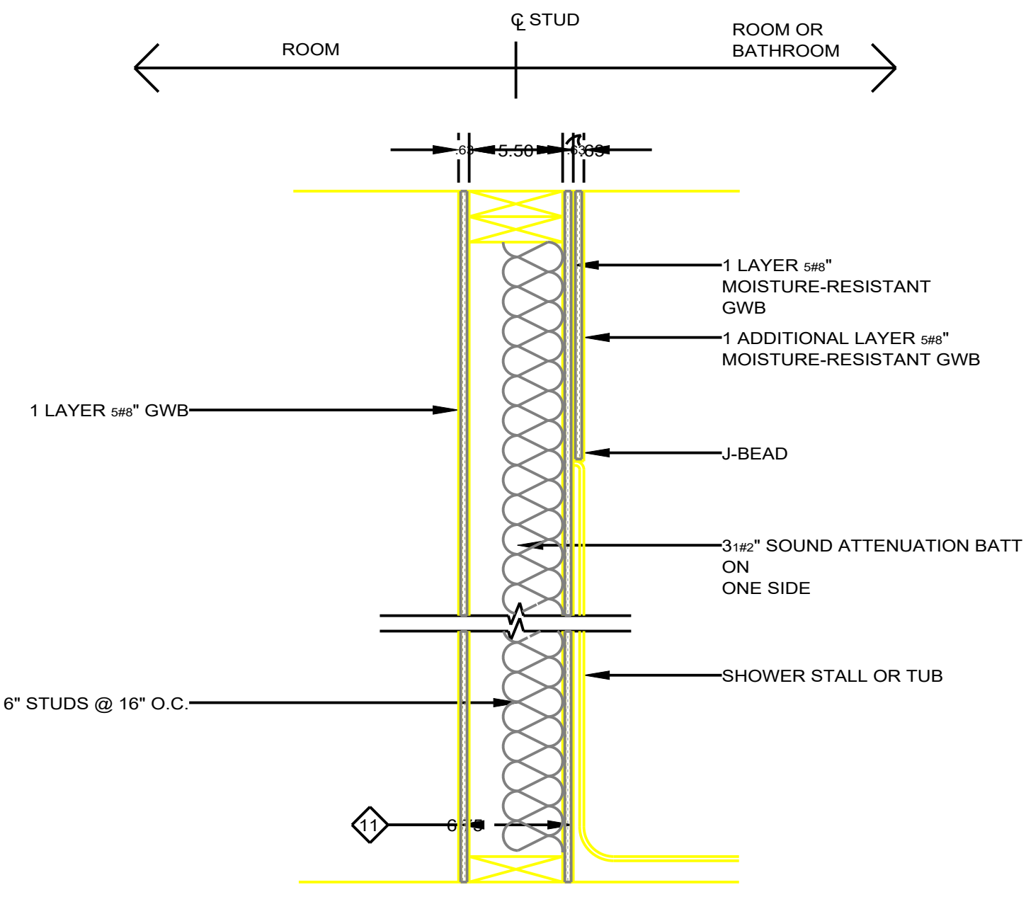
11 NON-RATED INTERIOR PARTITION
