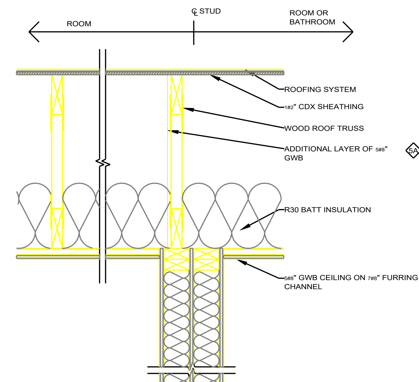
5 ONE HOUR RATED INTERIOR DEMISING PARTITION
