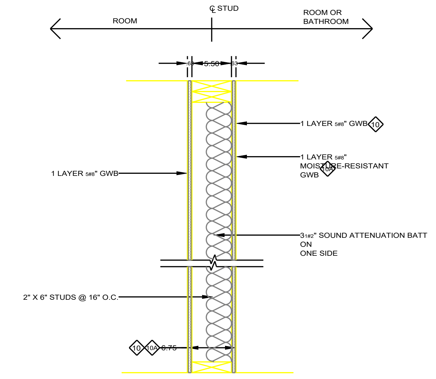
10 NON-RATED INTERIOR PARTITION
