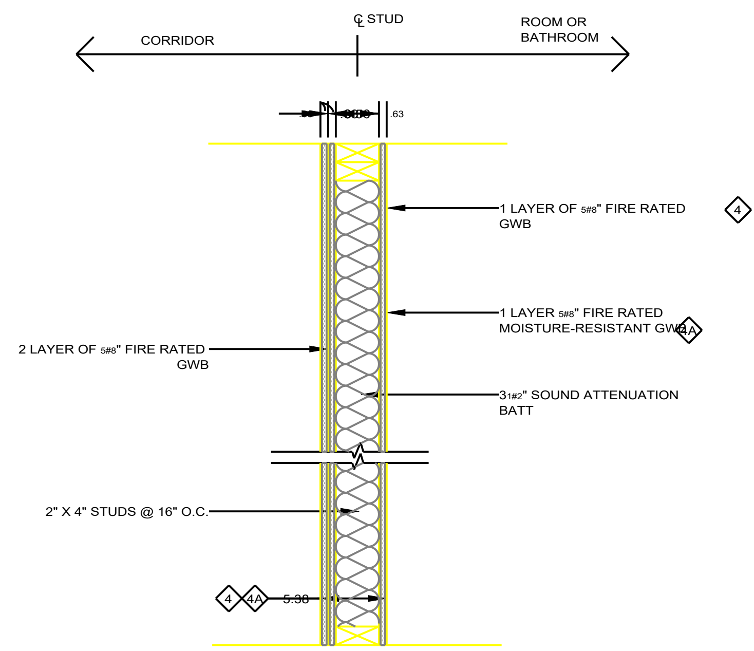
4 ONE HR RATED INTERIOR BEARING PARTITION
