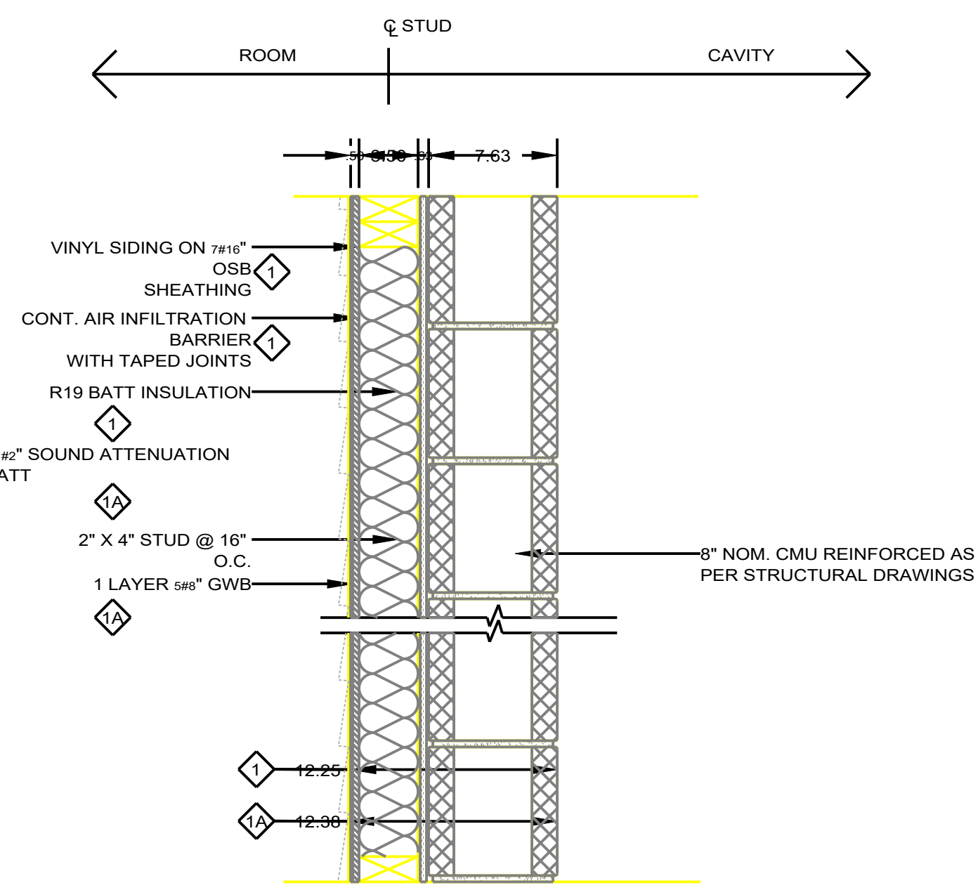
1 TWO HOUR RATED EXTERIOR BEARING FIRE
