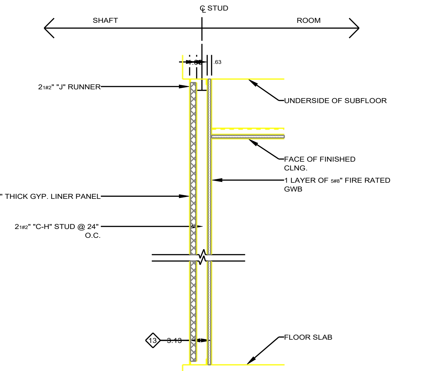
13 ONE HR RATED SHAFT WALL
