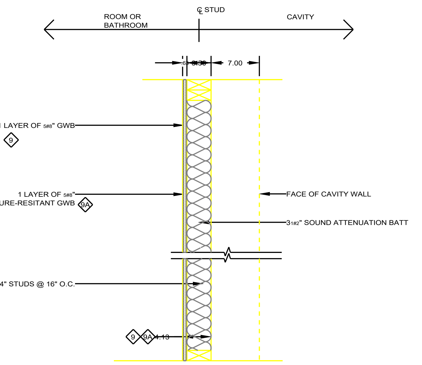
9 NON-RATED INTERIOR FURRING
