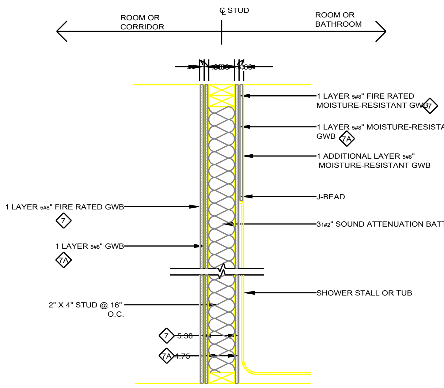
7 ONE HR RATED INTERIOR BEARING PARTITION
