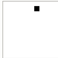
ch1 agent
