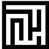
ch0 walls
