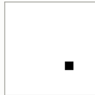
ch2 feature 0
