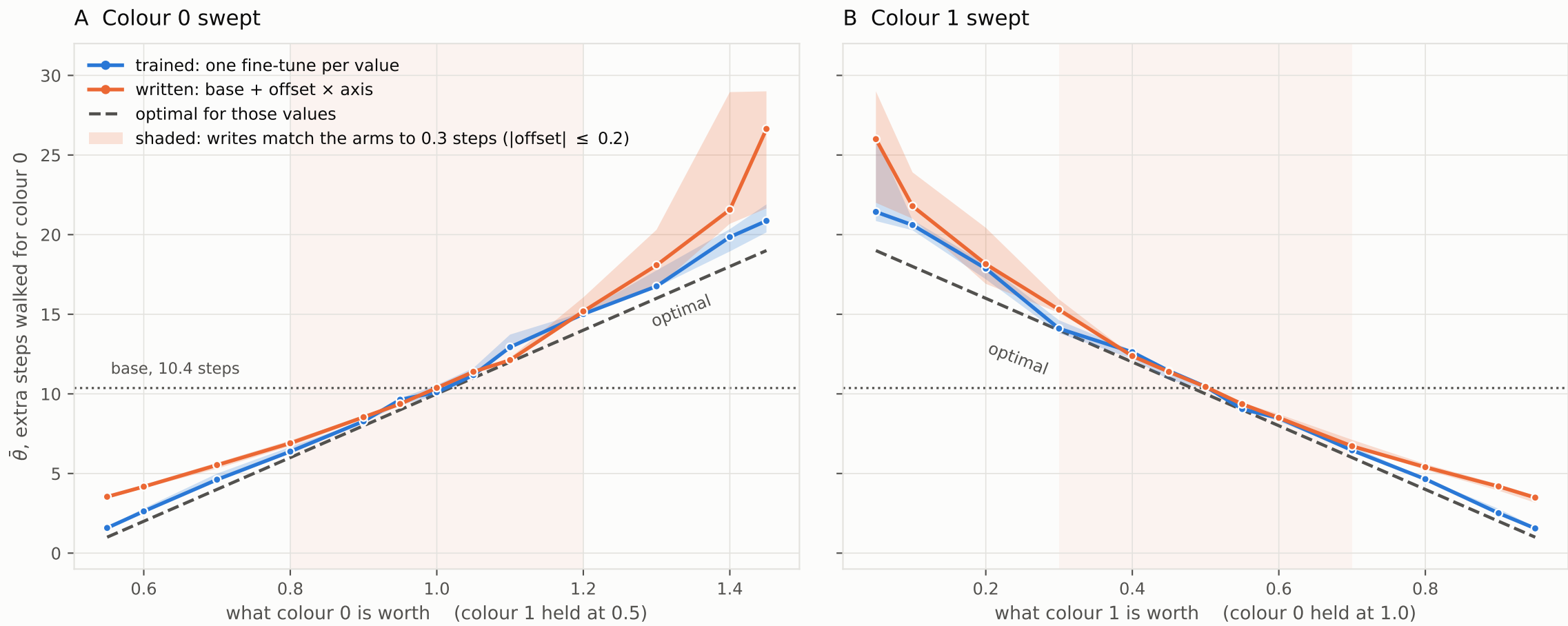
Figure 3 — One direction in weight space moves the threshold · bcnv11, 3 seeds, 20k held-out levels
