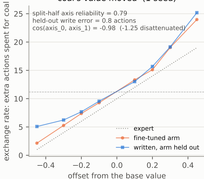
coal's value moved (1 seed)
