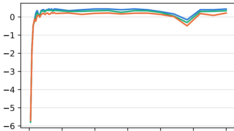
ResNet
