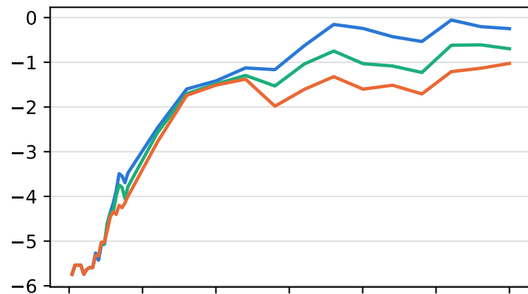
Transformer
