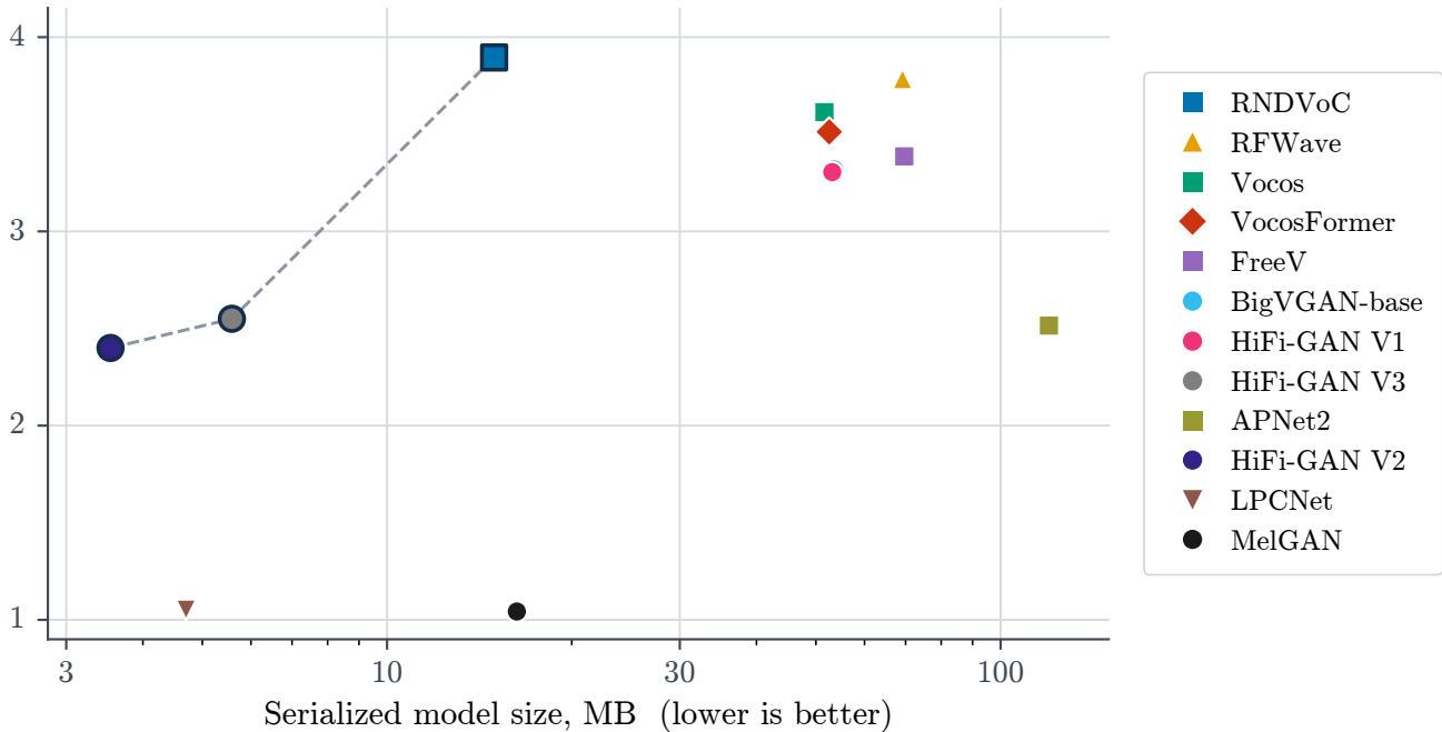
True-length wide-band PESQ (higher is better)
