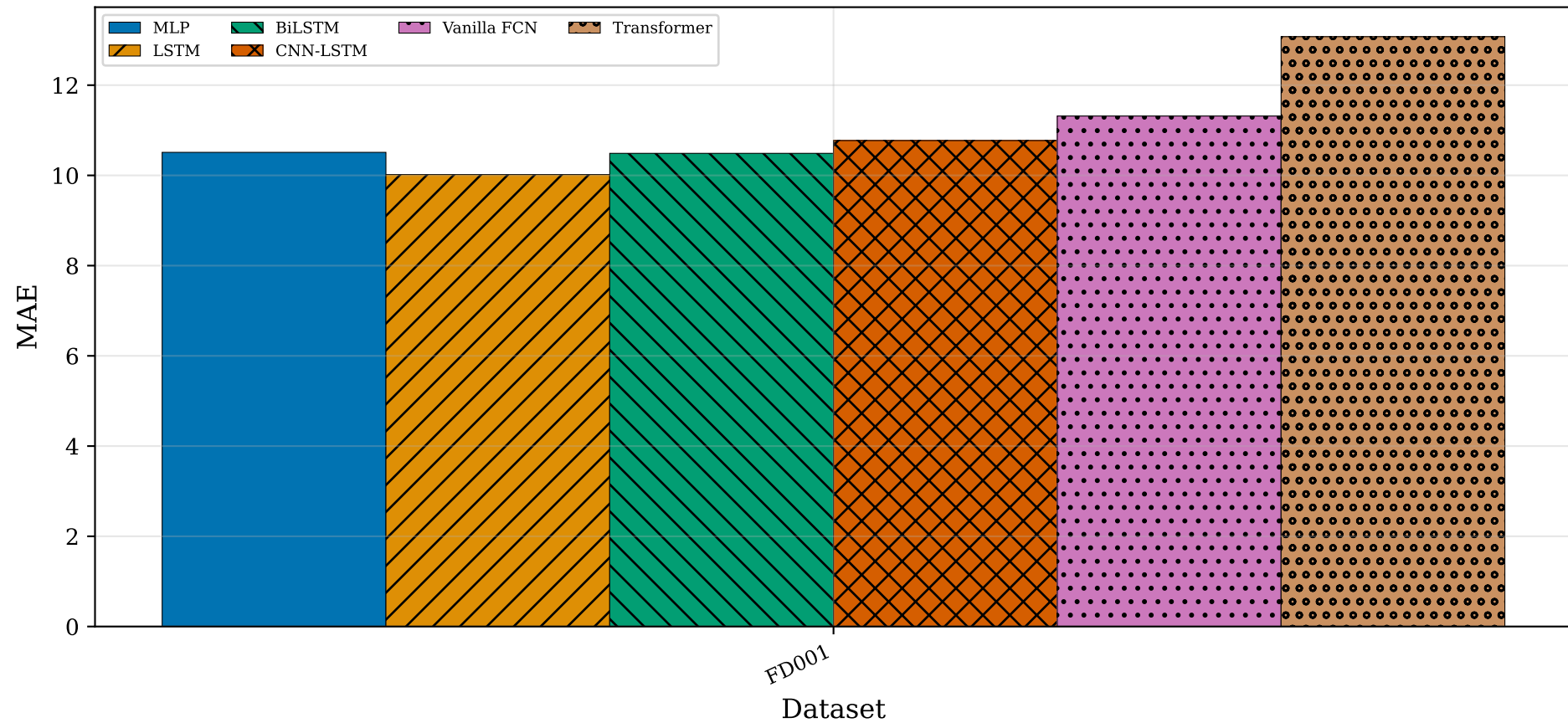
MAE — Baselines Comparison
