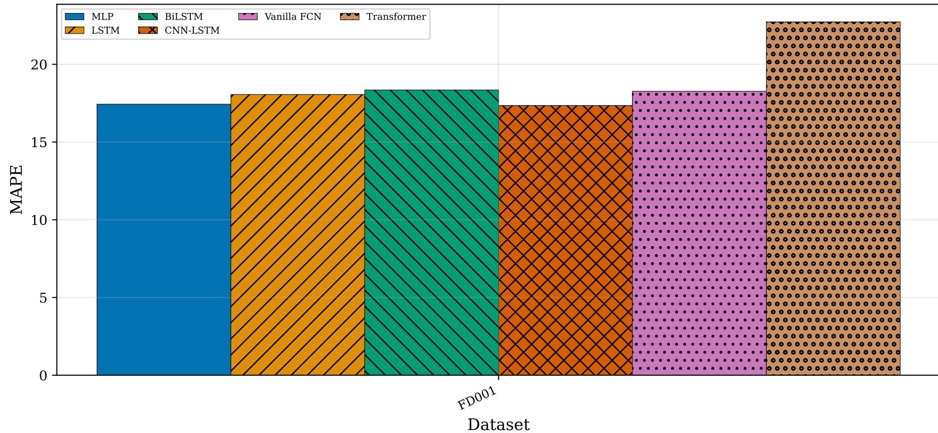
MAPE — Baselines Comparison
