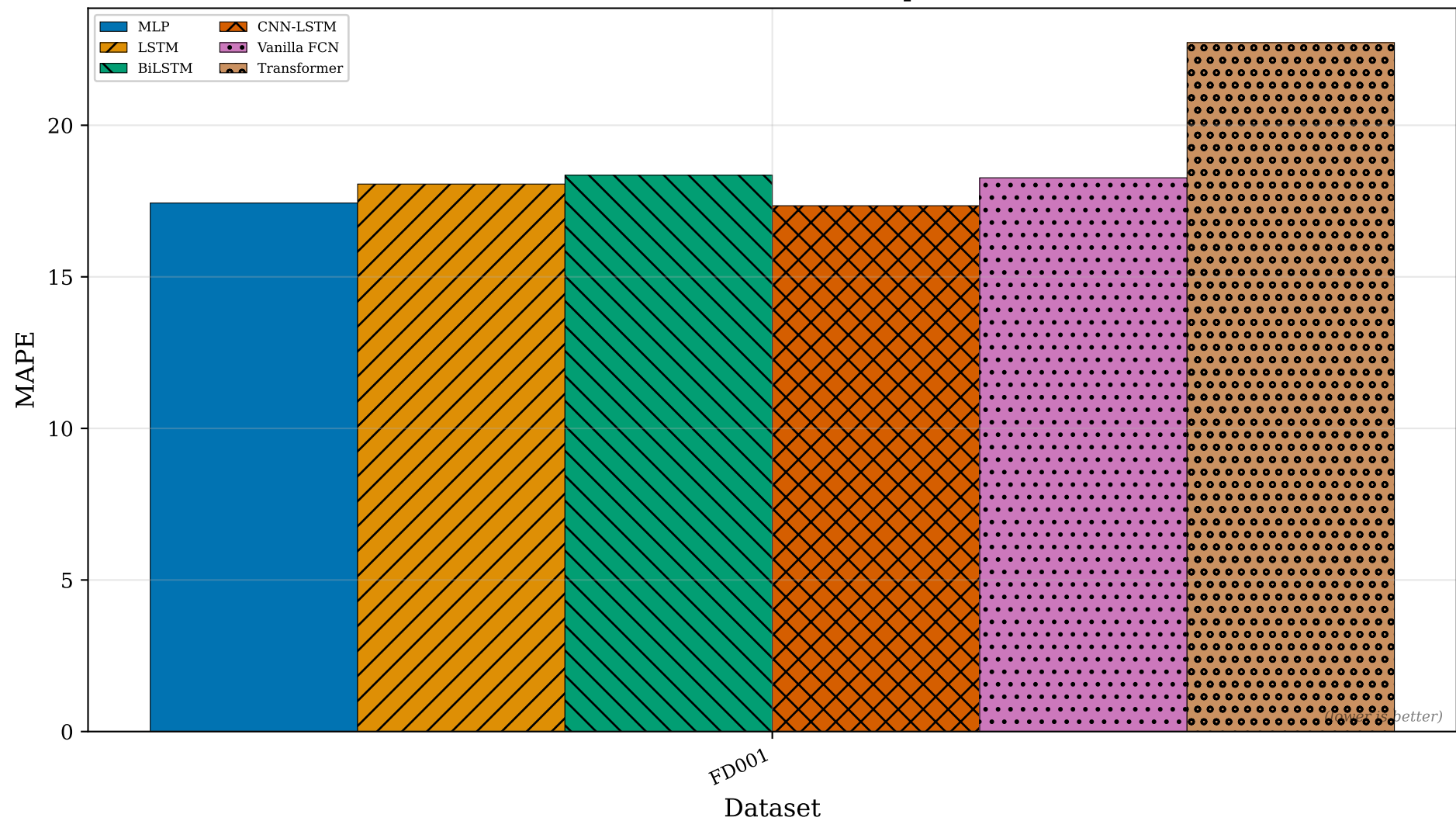
MAPE — All Methods Comparison
