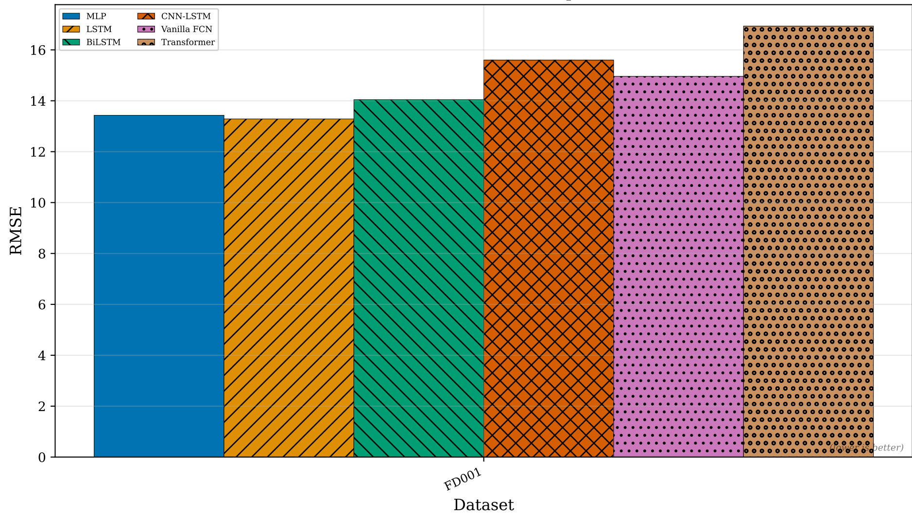
RMSE — All Methods Comparison
