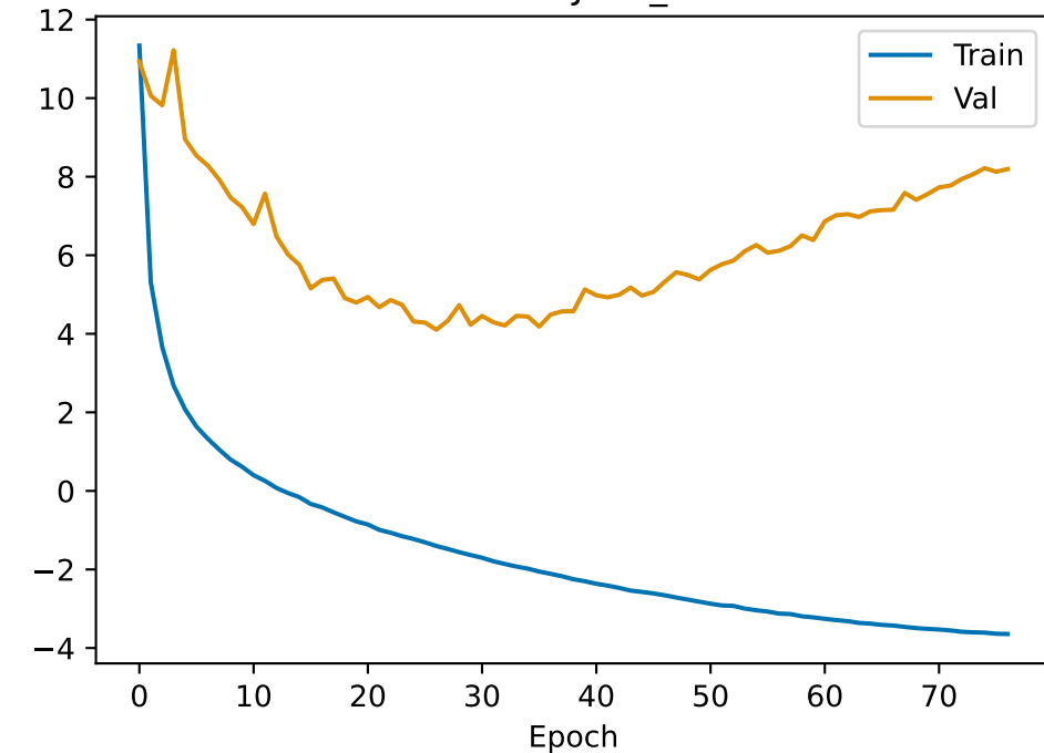
Total Loss — Jena_Climate
