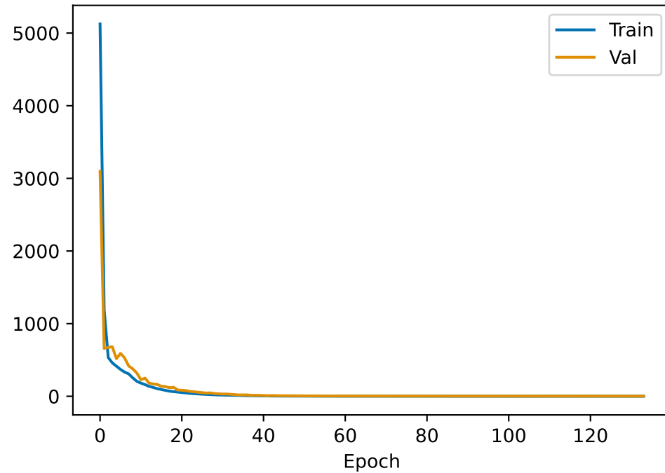
Total Loss — CMAPSS_FD001 (run 1)
