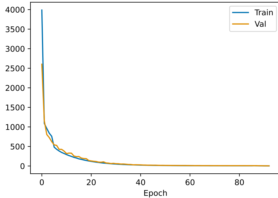
Total Loss — CMAPSS_FD002 (run 0)
