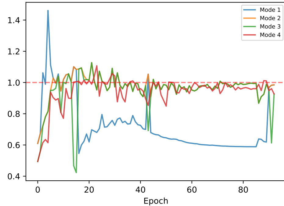
Koopman |\lambda|
