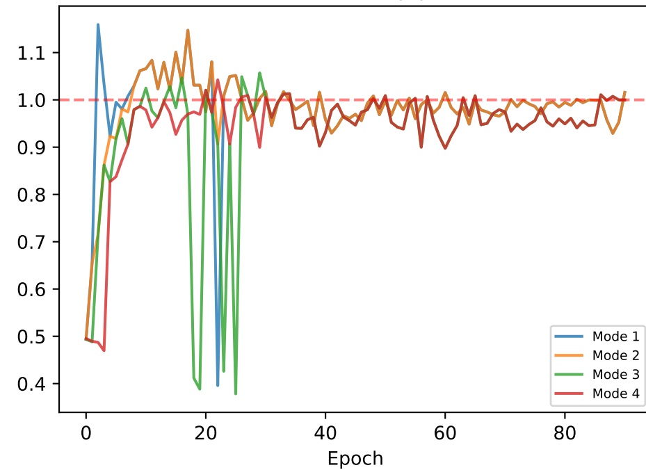
Koopman |\lambda|
