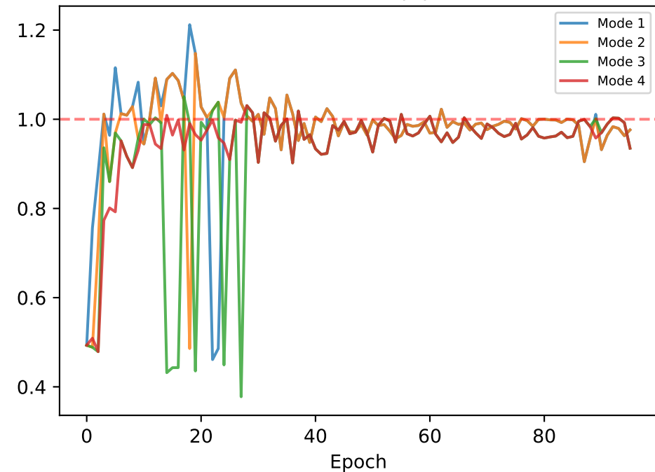
Koopman |\lambda|
