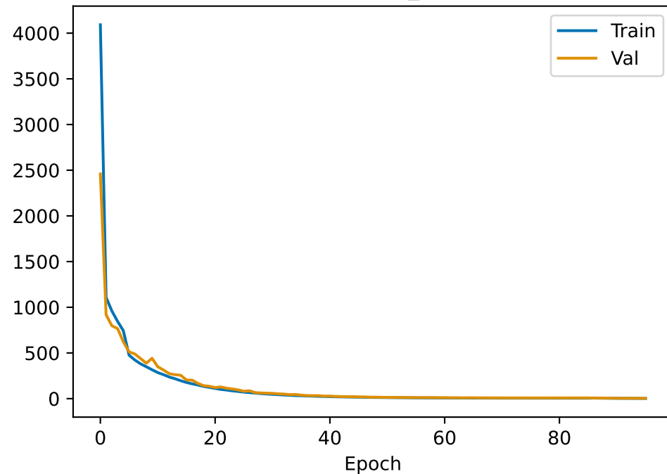
Total Loss — CMAPSS_FD002 (run 2)
