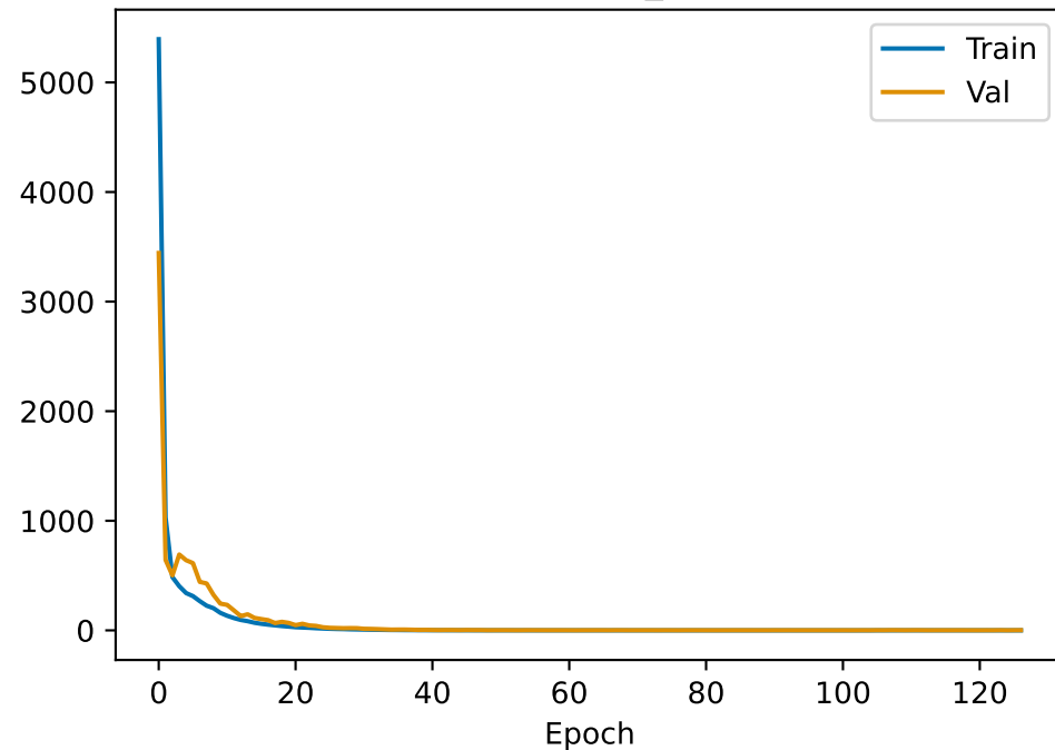
Total Loss — CMAPSS_FD003 (run 1)
