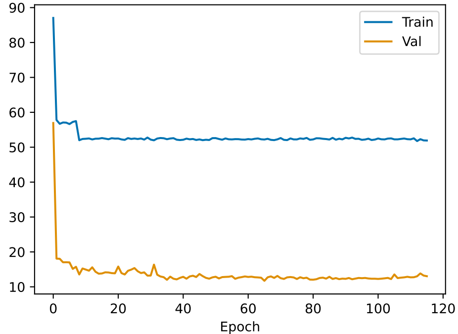
RMSE
