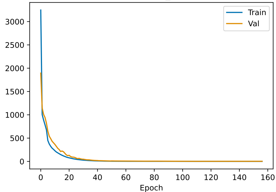
Total Loss — CMAPSS_FD004 (run 0)
