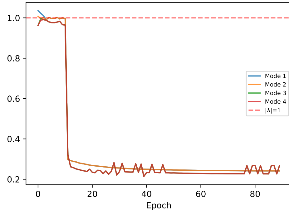
Koopman |\lambda| Evolution
