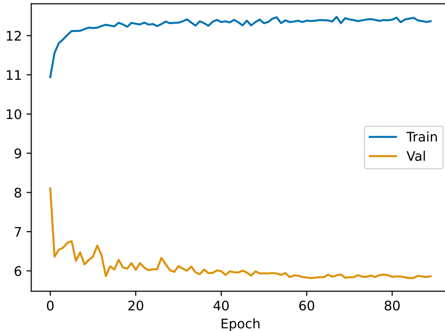
RMSE
