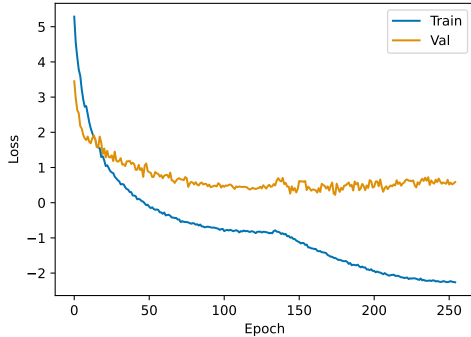
Total Loss — SPY_Stock
