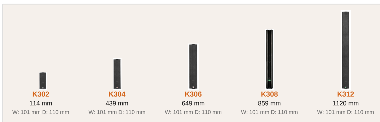
Figure 2 – K-Series models shown proportionally to relative height. All models: 101 mm wide × 110 mm deep.
