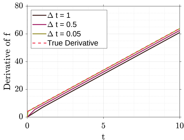
Figure 2: Discrete Derivative and Sampling Time.
