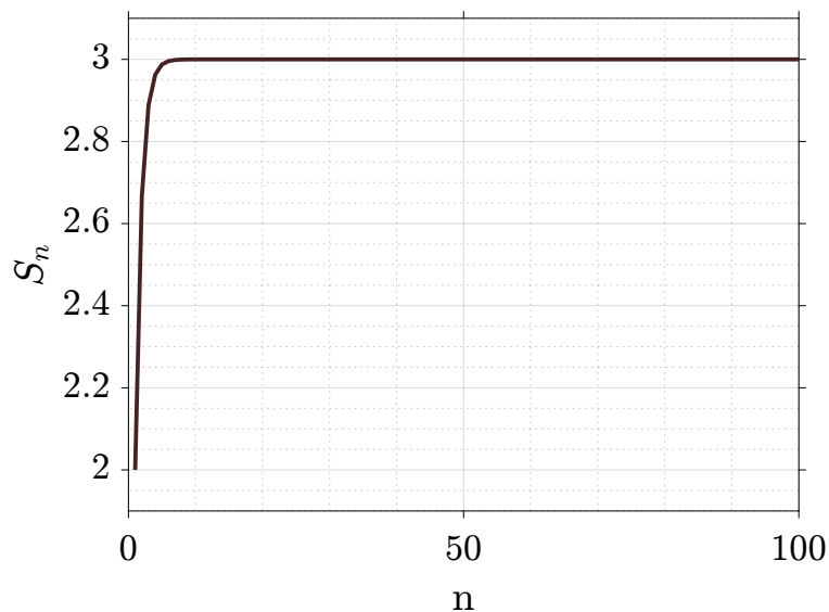
Figure 1: Convergence of a Geometric Progression.
