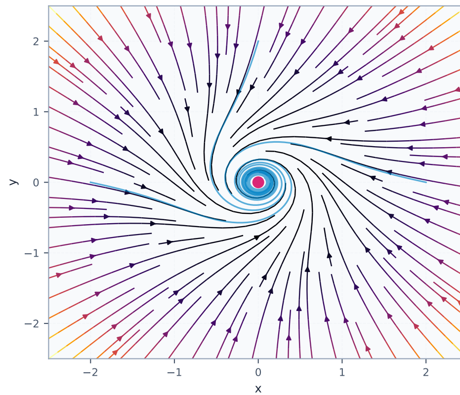
Hopf Bifurcation \mu = 0 (centre)
