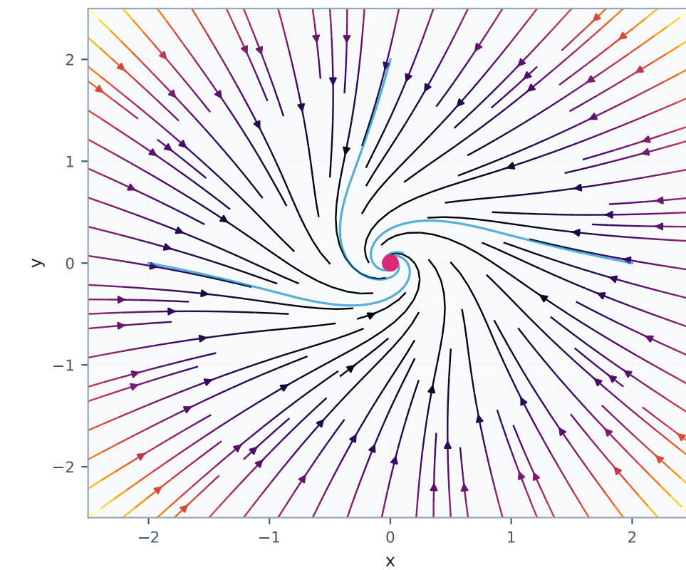
Hopf Bifurcation \mu = -0.5 (stable spiral)
