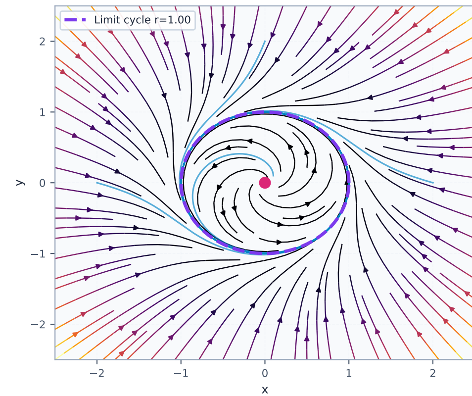
Hopf Bifurcation \mu = 1 (limit cycle)
