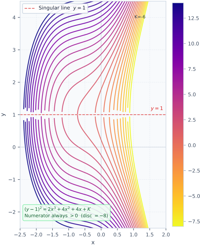
Solution Family: (y - 1)^2 = 2x^3 + 4x^2 + 4x + K
