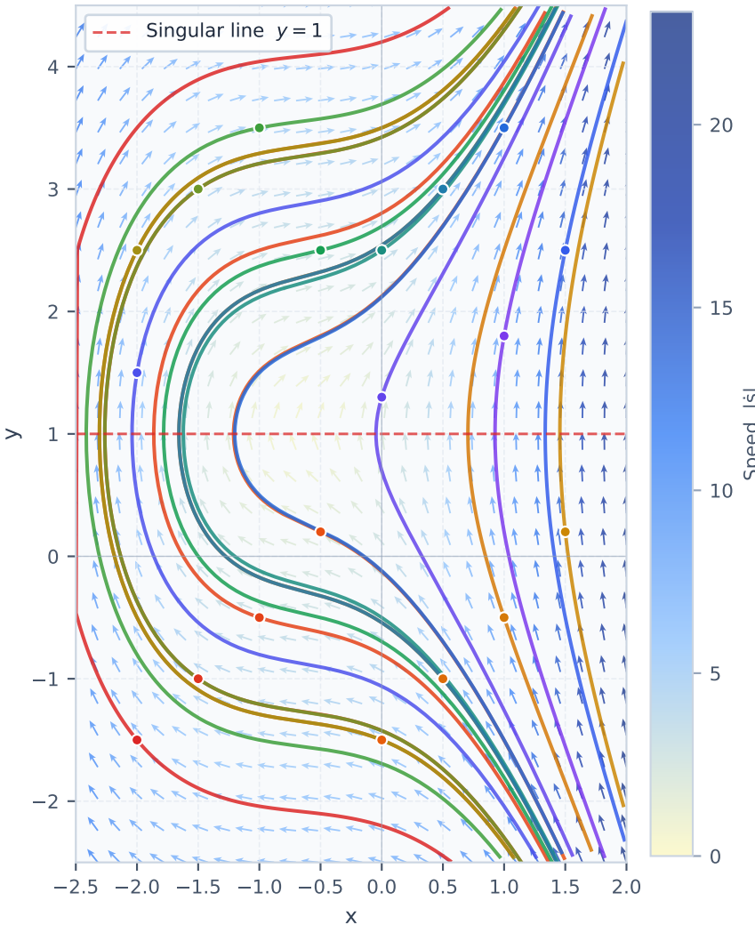
Phase Portrait — Vector Field & Integral Curves
