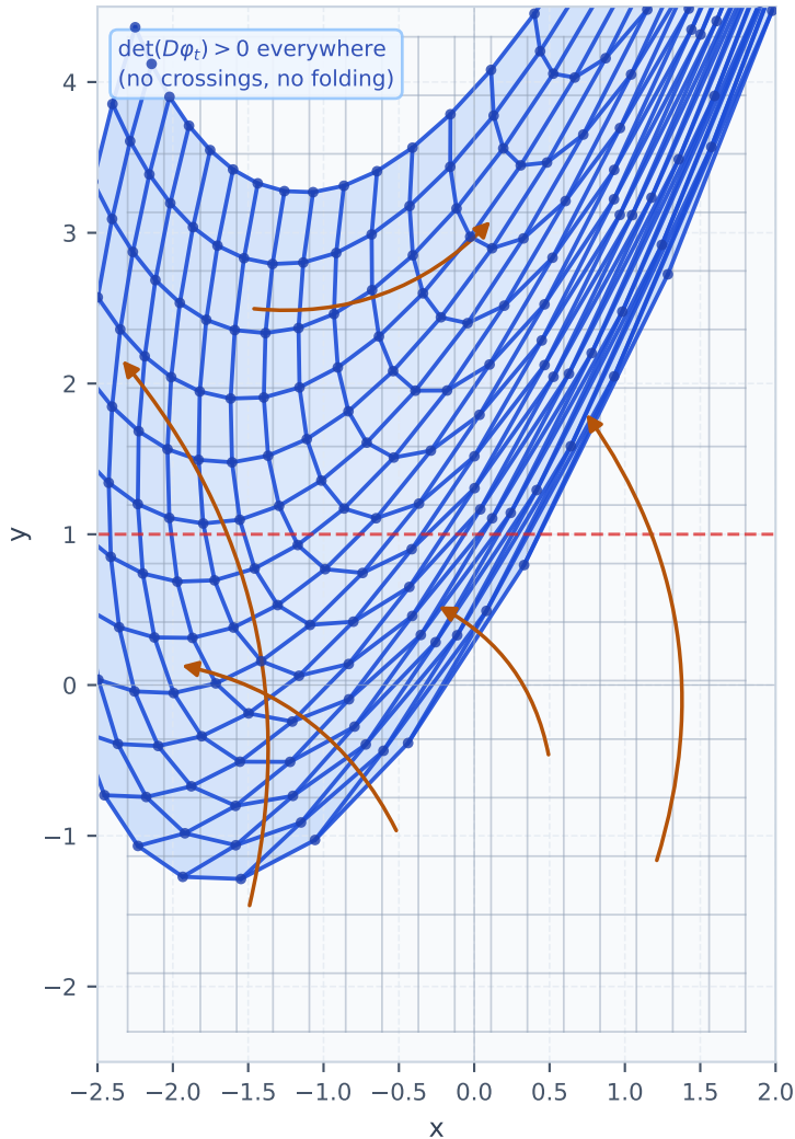
Deformed Grid — Diffeomorphism \varphi_t ( t = 0.45 )
