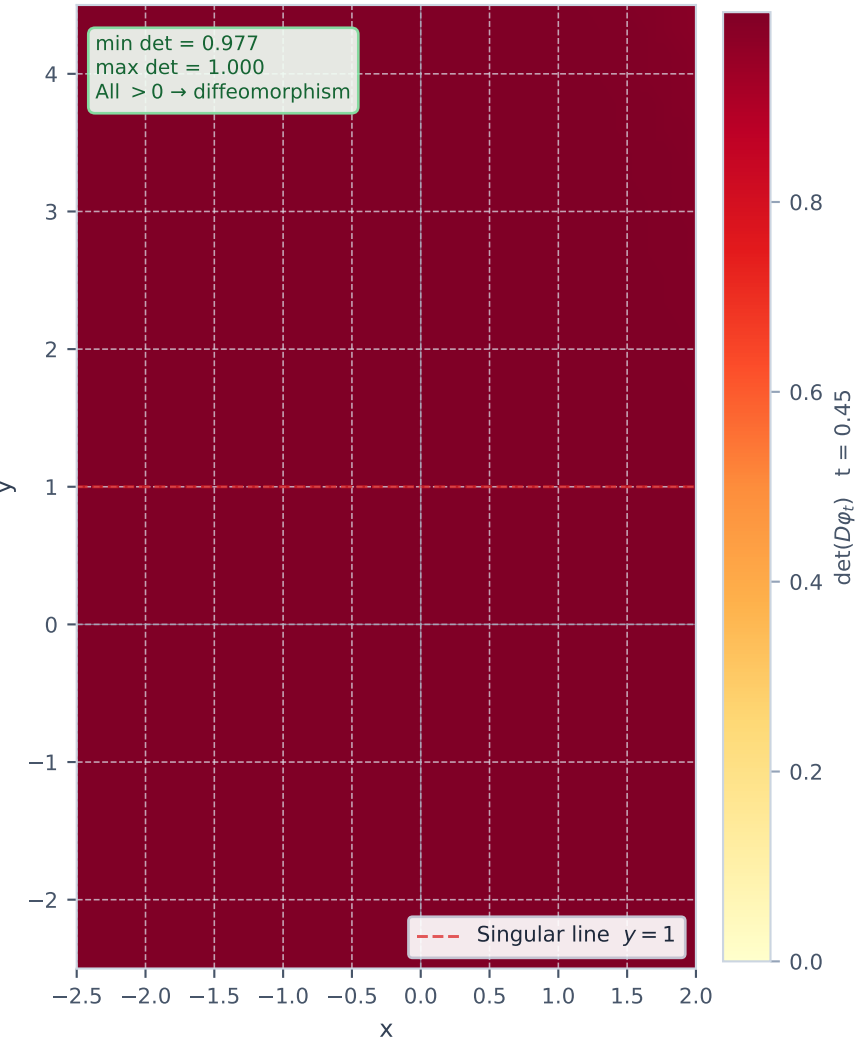
Jacobian \det(D\varphi_t) — Confirms Diffeomorphism
