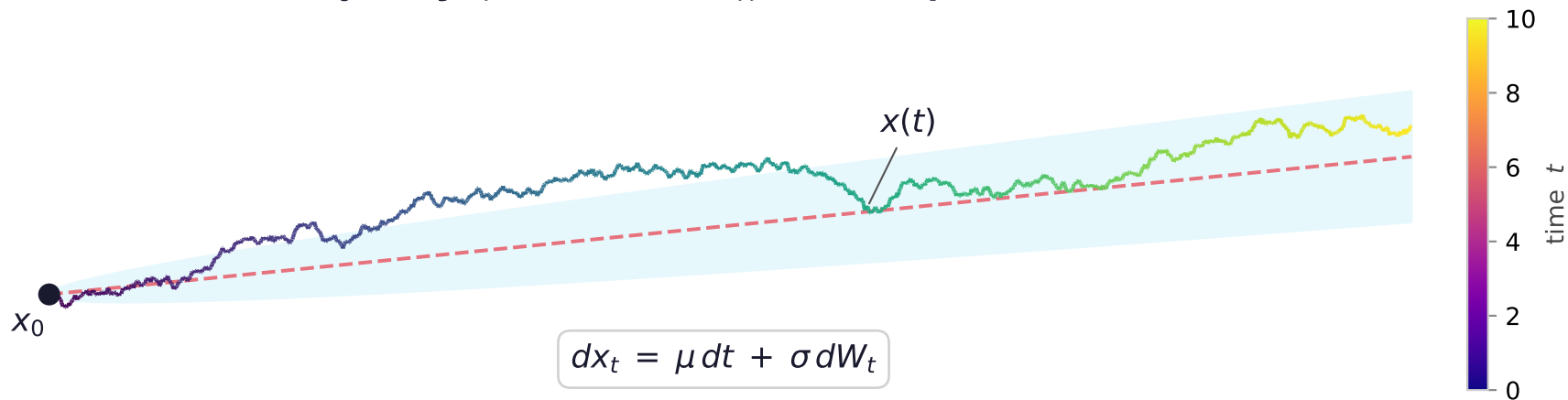
Trajectory of a stochastic differential equation (SDE)
