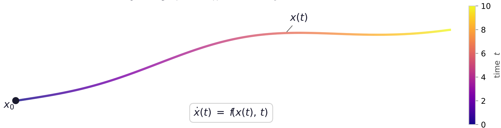
Trajectory of the differential equation (ODE)
