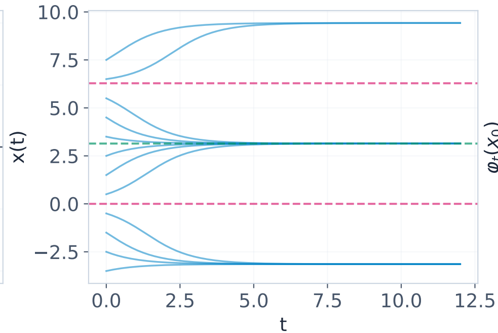
Solution Curves x(t)
