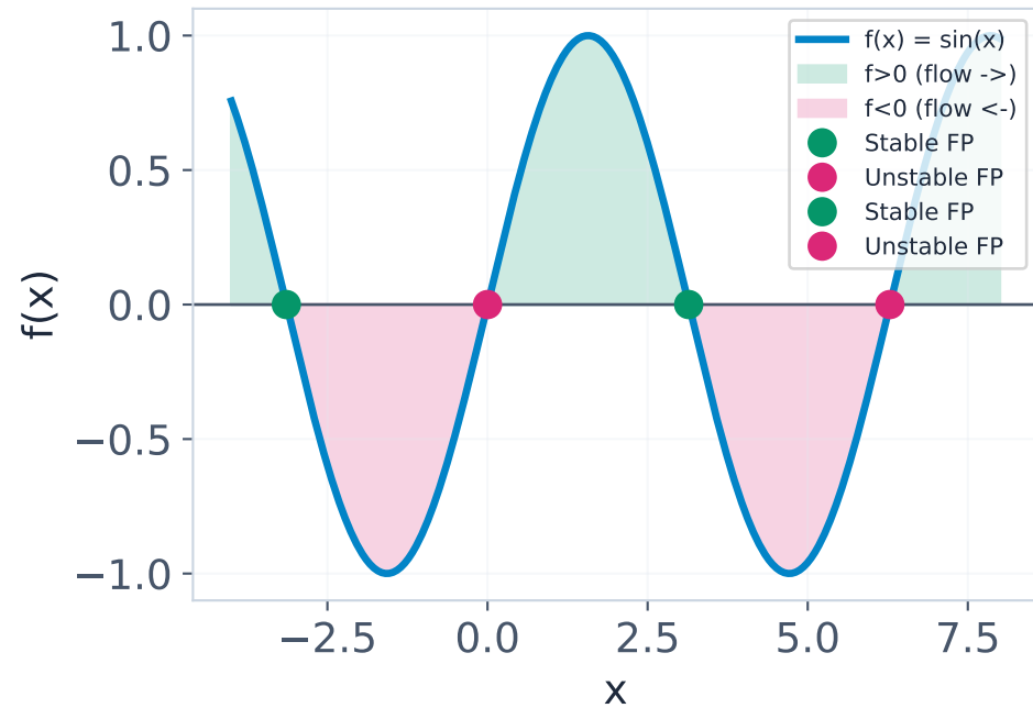
Phase Line (1-D)
