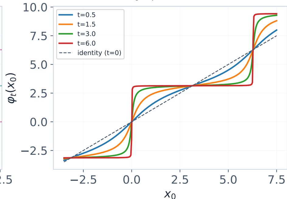
Flow Map \varphi_t(x_0) at various t
