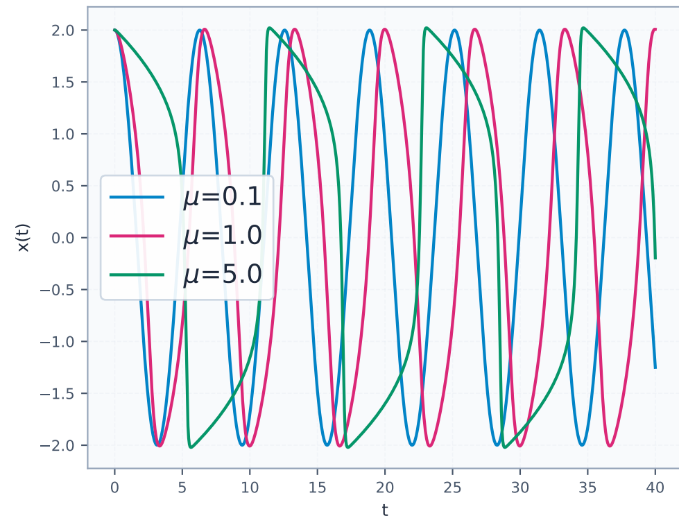
Time Series x(t) for \mu = 0.1, 1, 5
