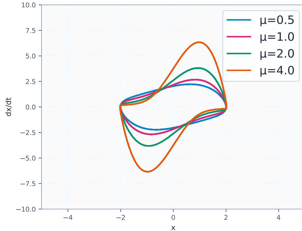
Limit Cycles for \mu = 0.5, 1, 2, 4
