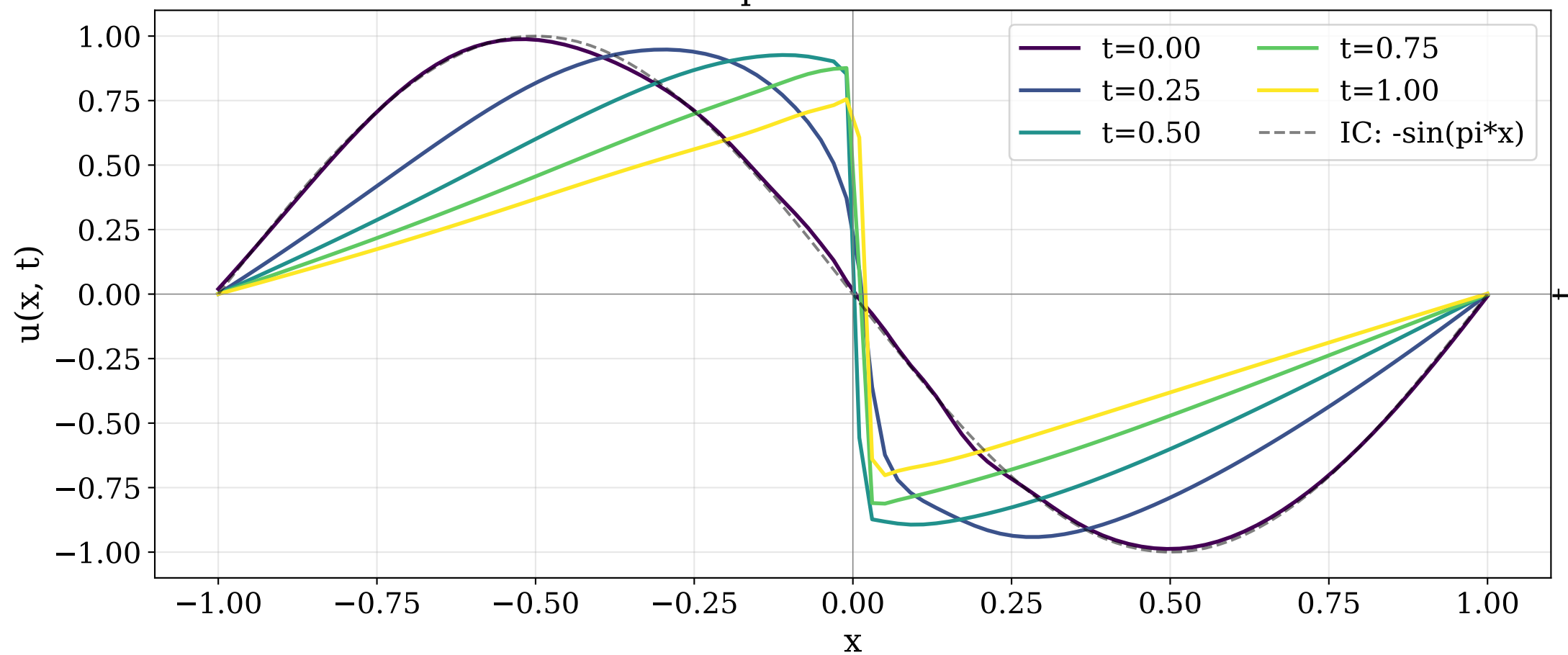
Solution profiles at fixed times
