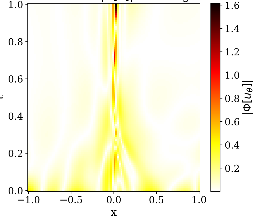
PDE residual |\Phi[u]| on eval grid
