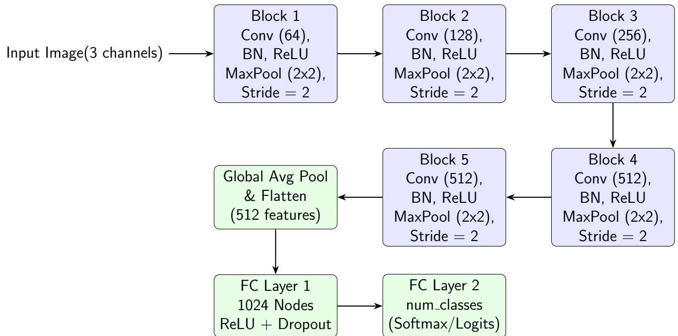
Figure 1: CNN Architecture, BN means Batch Normalization, FC means fully connected layer. Global average pooling can be implemented using nn.AdaptiveAvgPool2d
