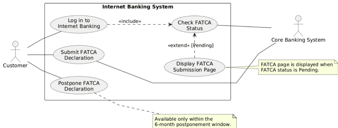
Figure 1: FATCA declaration use case diagram
