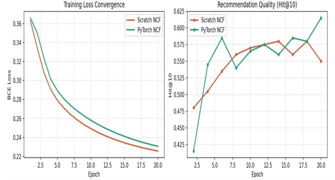
Fig. 2. Extended convergence analysis over the full 20-epoch training run, showing BCE loss (left panel) and Hit@10 quality (right panel) for both implementations simultaneously. The parallel convergence trajectories confirm implementation equivalence.
