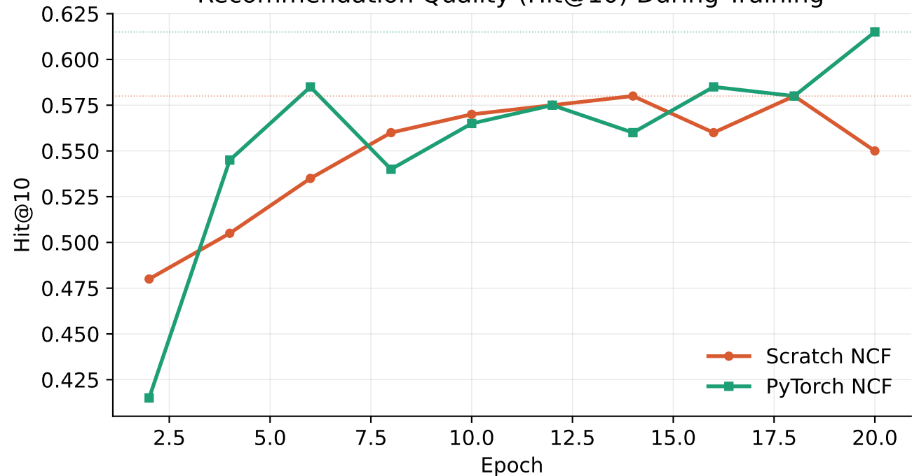
Recommendation Quality (Hit@10) During Training
