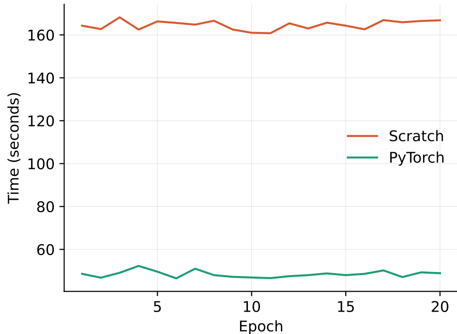
Per-Epoch Training Time
