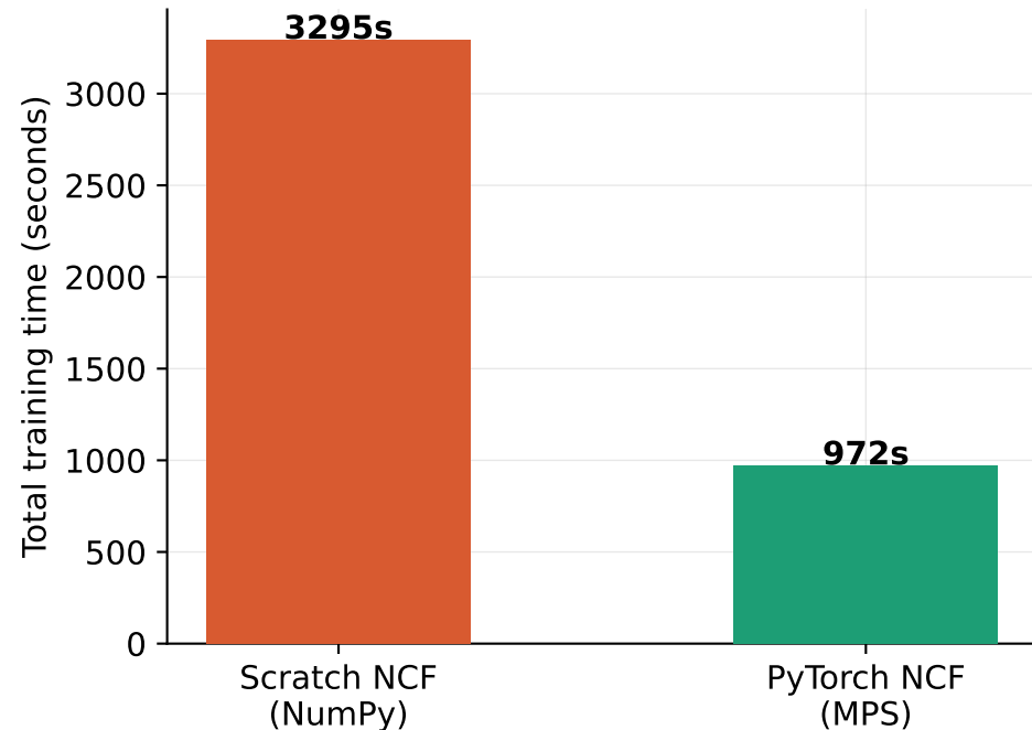
Training Efficiency (3.39× speedup)
