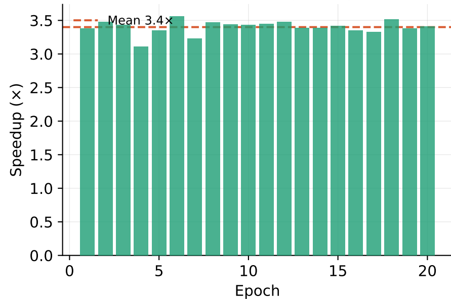
(C) Per-epoch speedup
