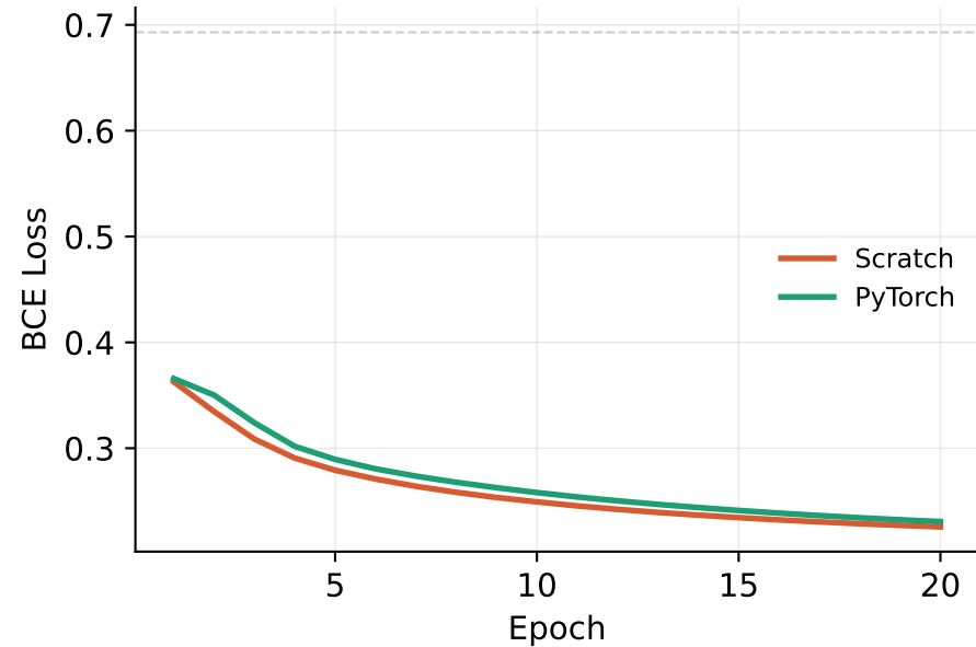
(A) Loss convergence
