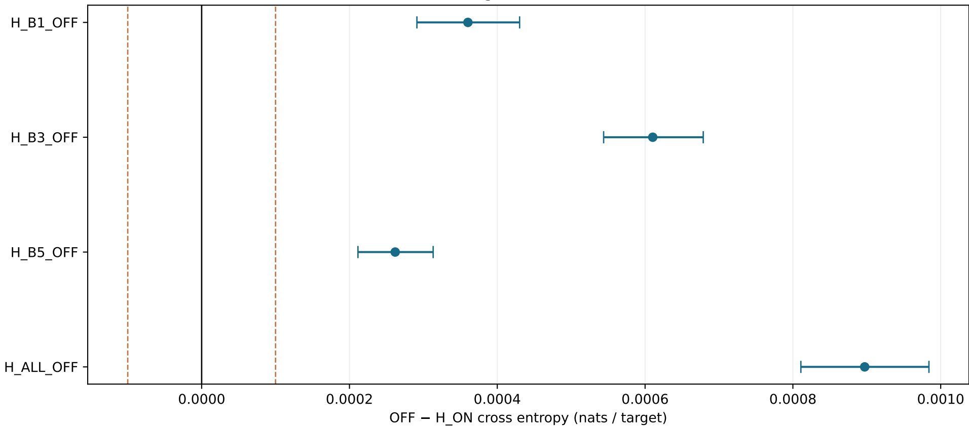
H10B recurrence removal · paired sequence bootstrap 98.75% Bonferroni marginal intervals; reference \pm 0.0001
