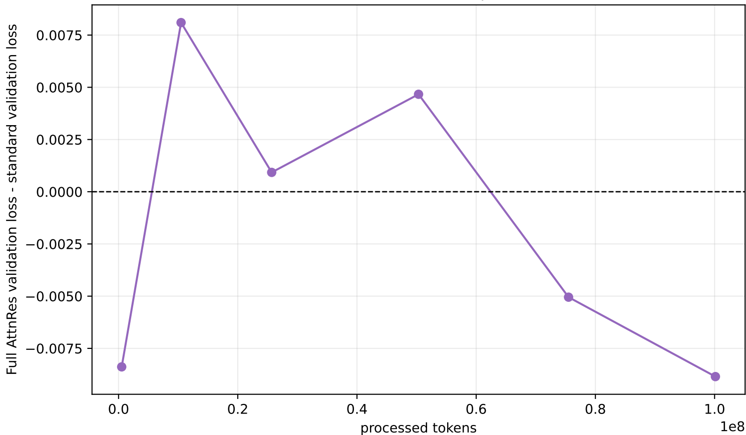
Matched validation-loss delta vs processed tokens
