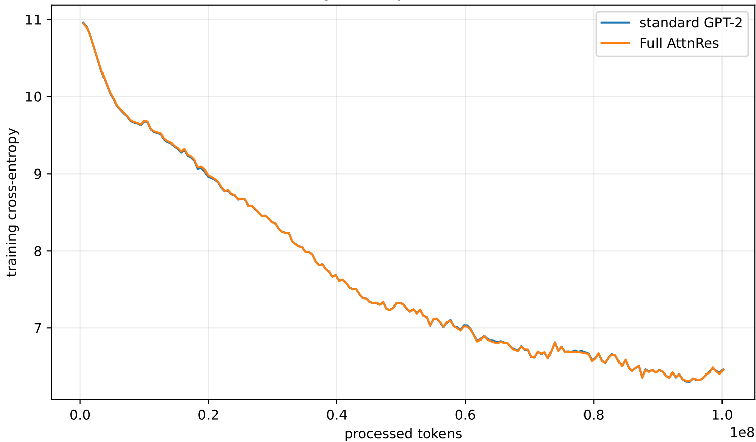
Training loss vs processed tokens
