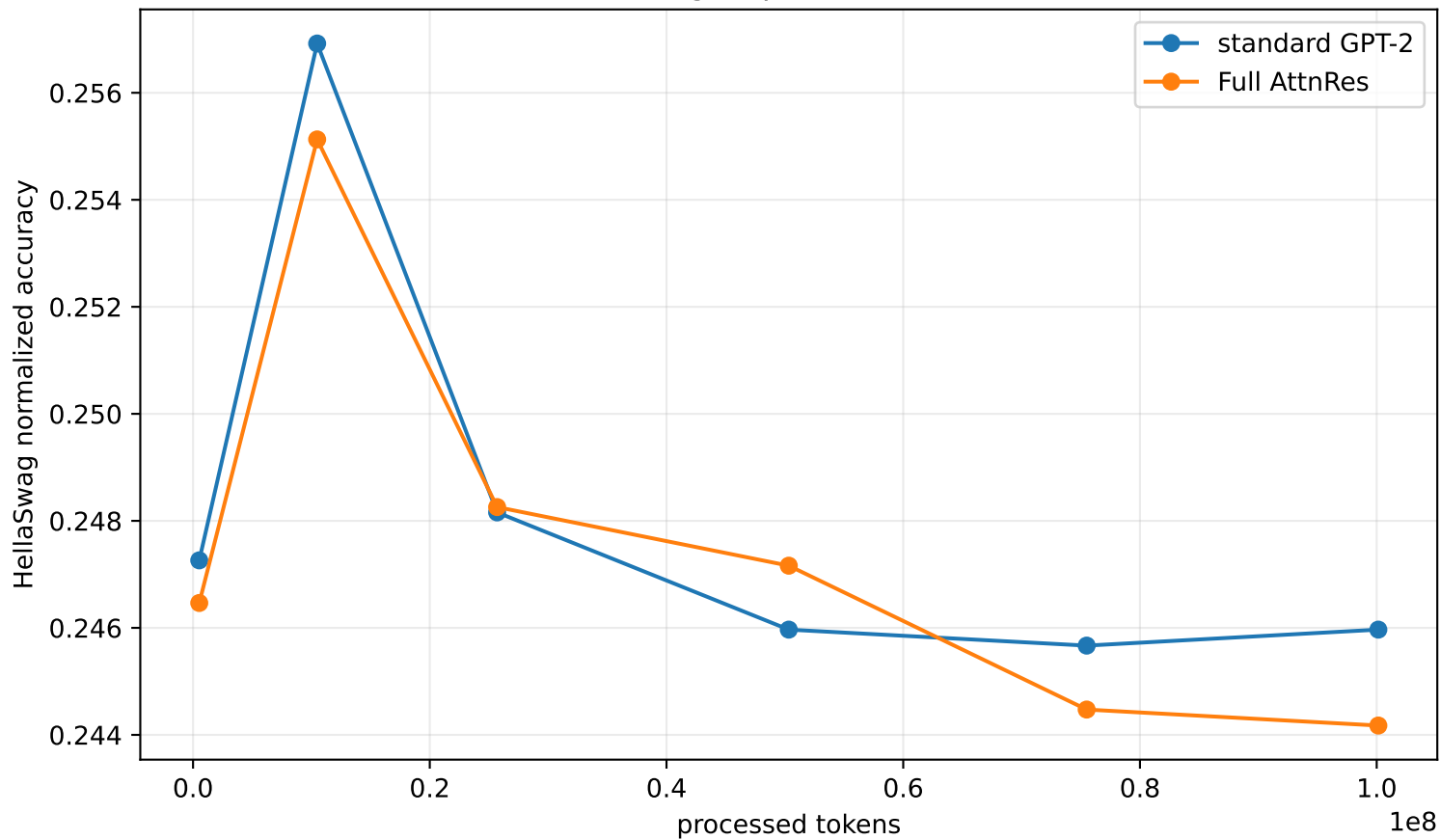
HellaSwag vs processed tokens
