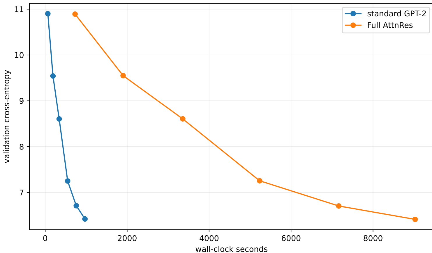
Validation loss vs wall-clock time
