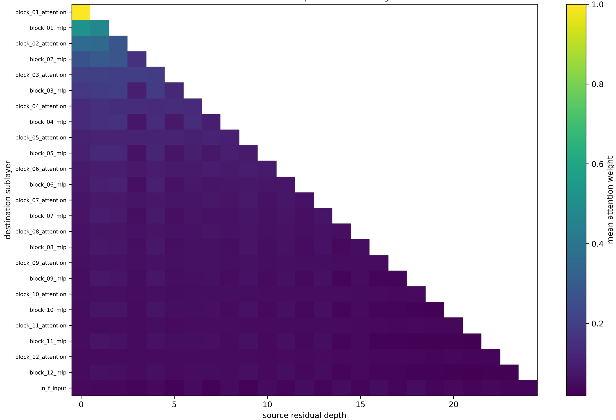
Full AttnRes mean depth-attention weights
