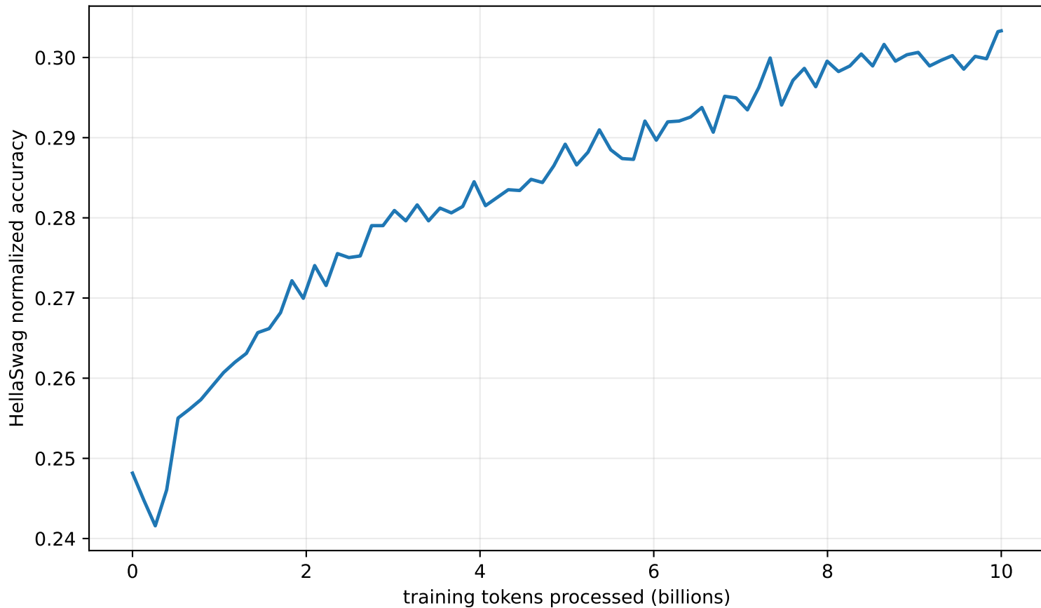
HellaSwag accuracy
