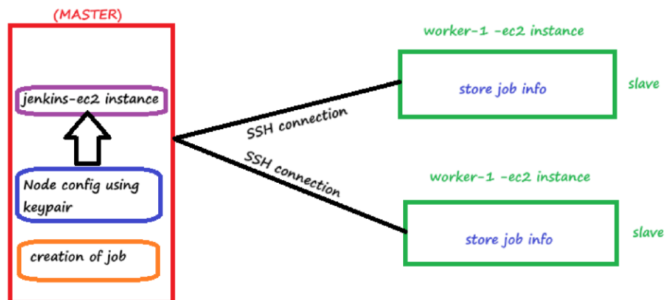
Master and slave architecture in Jenkins
