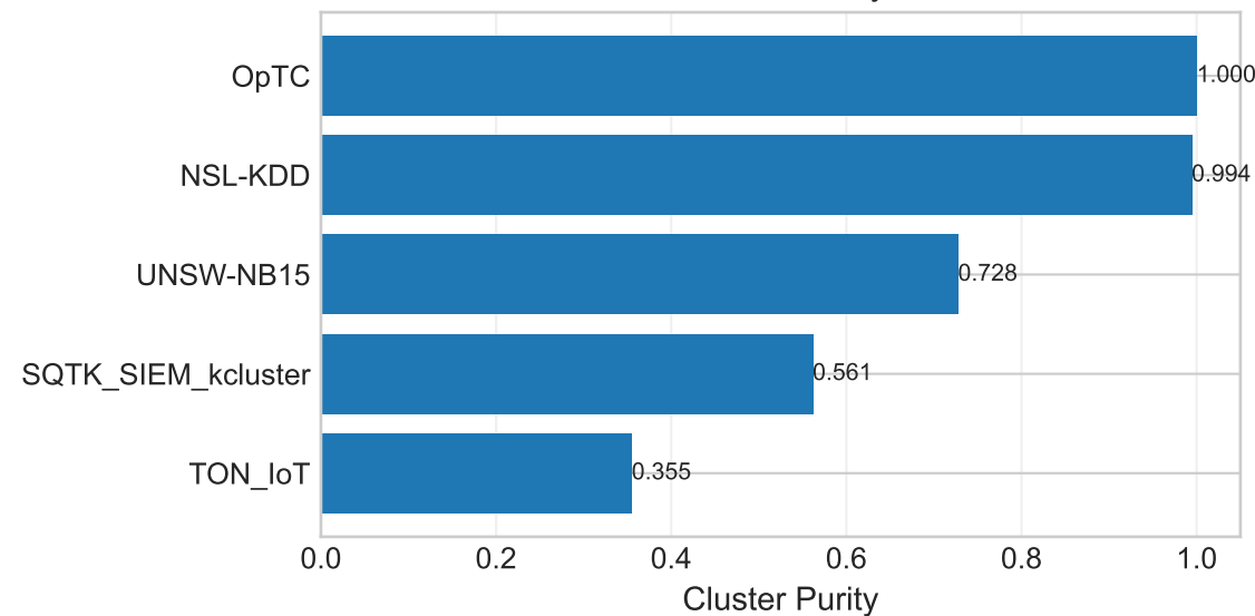
Cluster Purity
