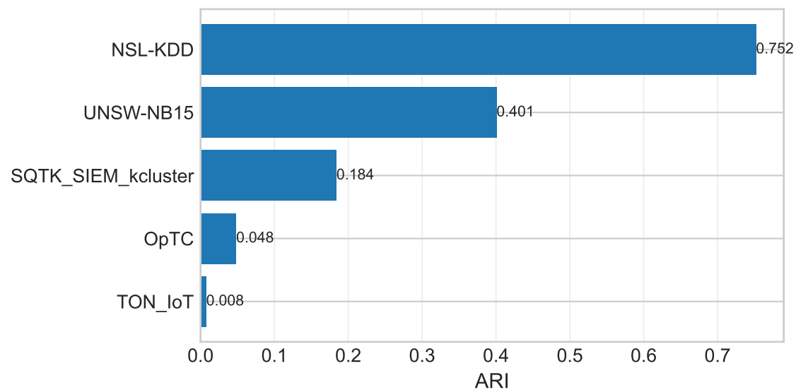
ARI
