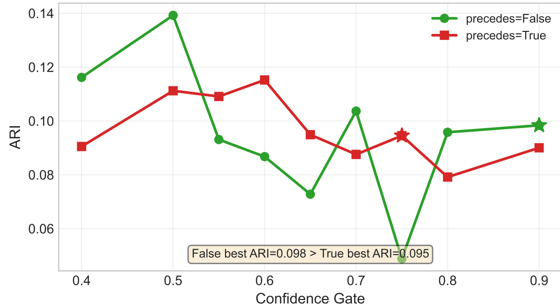
ARI: TON_IoT
