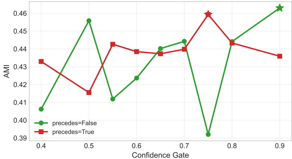
AMI: TON_IoT
