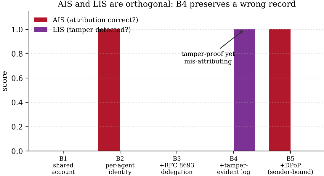
Figure 2: AIS and LIS per baseline. Only B4 carries a hash-chained log, so only B4 reaches \text{LIS} = 1.0 ; yet B4’s AIS is 0.0 — the tamper-evident log preserves the wrong record. Generated from the live harness.
