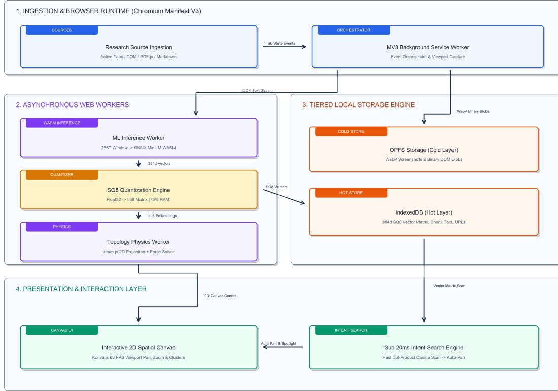
Figure 3: Meridian End-to-End System Architecture: decoupled Chromium MV3 runtime with dedicated ML Web Workers, tiered local storage, and high-performance Konva.js 2D spatial canvas.
