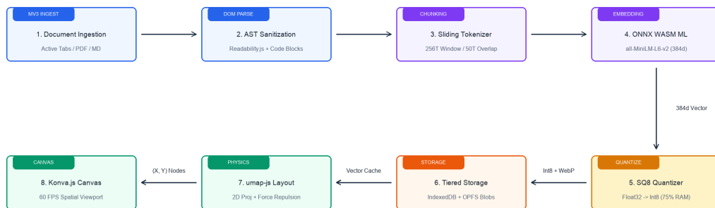
Figure 1: Squarish Pipeline Architecture: Modular tree-fork flow showing DOM sanitization, sliding-window chunking, on-device WASM embedding, SQ8 quantization, and 60 FPS canvas projection.
