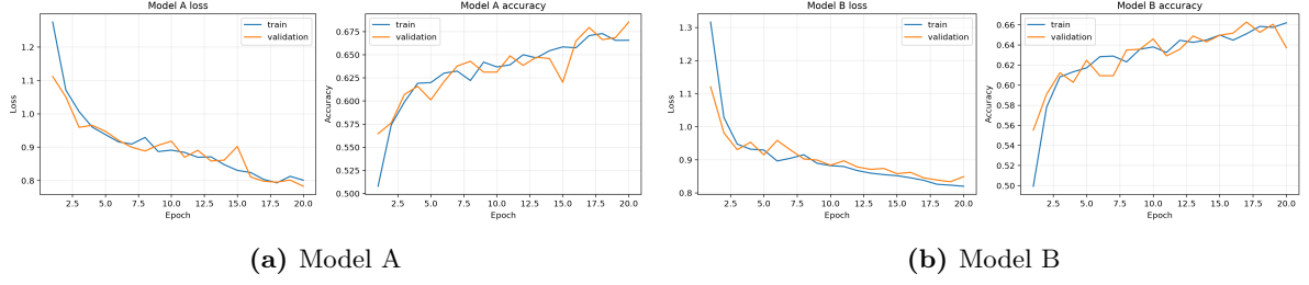
Figure 3: Training and validation curves for the custom CNNs.
