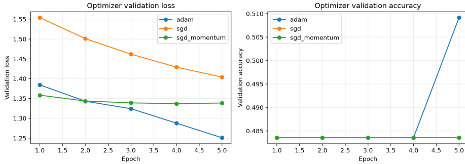
Figure 2: Optimizer pilot curves generated from the saved optimizer comparison artifact.
