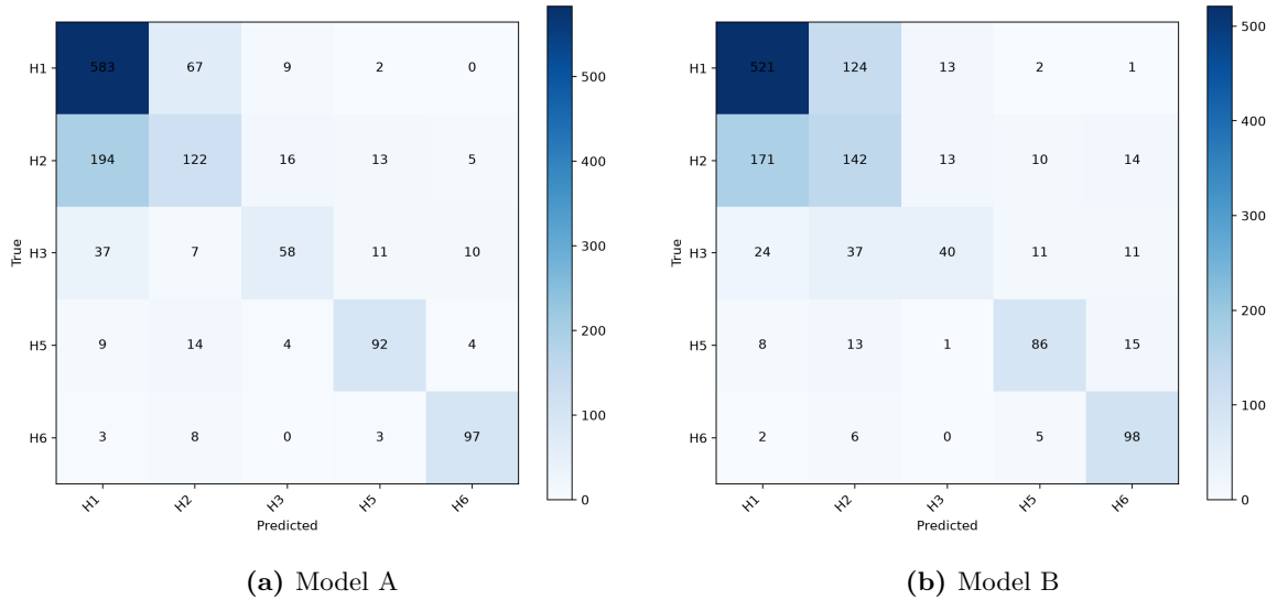
Figure 4: Verified custom CNN confusion matrices on the canonical test set.
