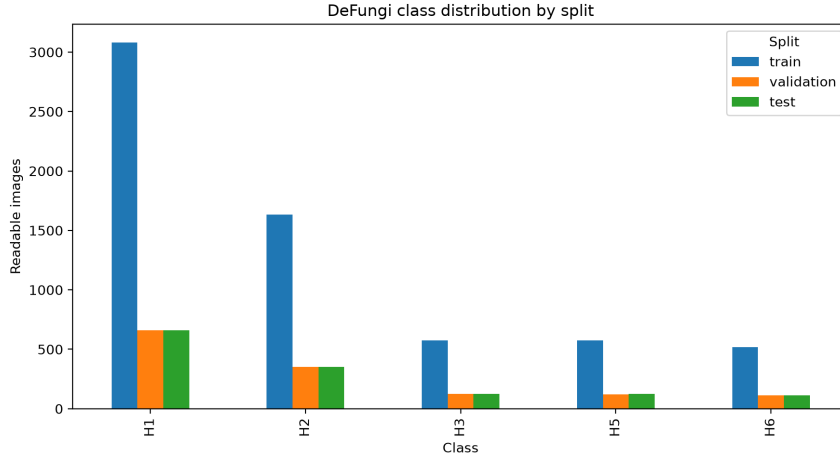
Figure 1: Verified class distribution generated from the saved dataset summary.
