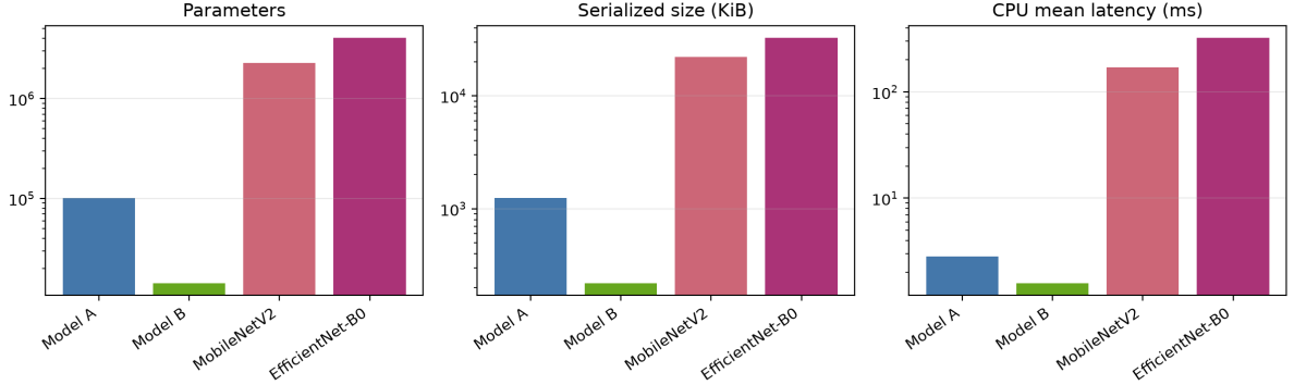
Figure 8: Final resource comparison. The y-axes are logarithmic to show custom and pretrained models in one figure.
