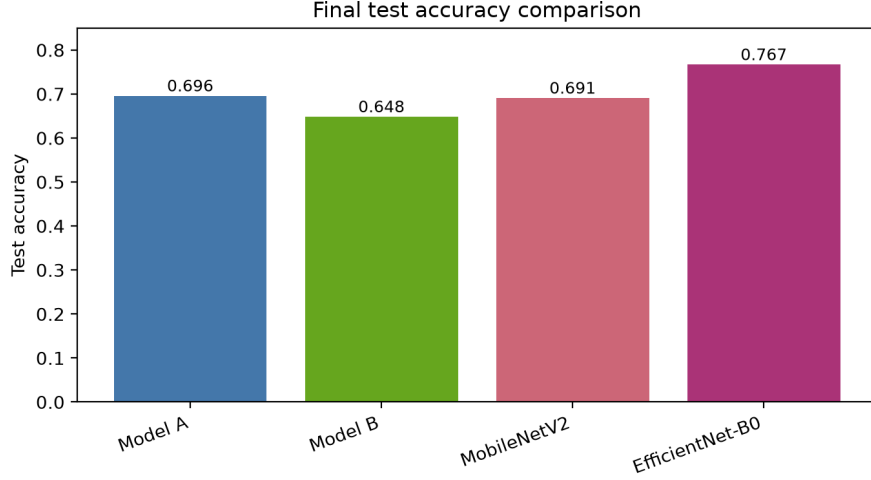
Figure 7: Final test accuracy comparison from the verified final comparison CSV.
