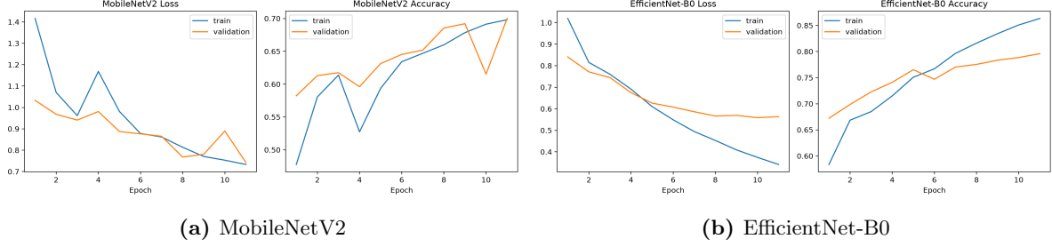
Figure 5: Training and validation curves for the 64×64 transfer-learning runs.
