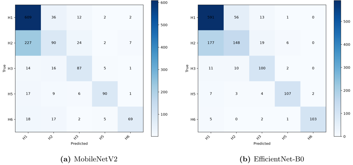
Figure 6: Verified transfer-learning confusion matrices on the canonical test set.
