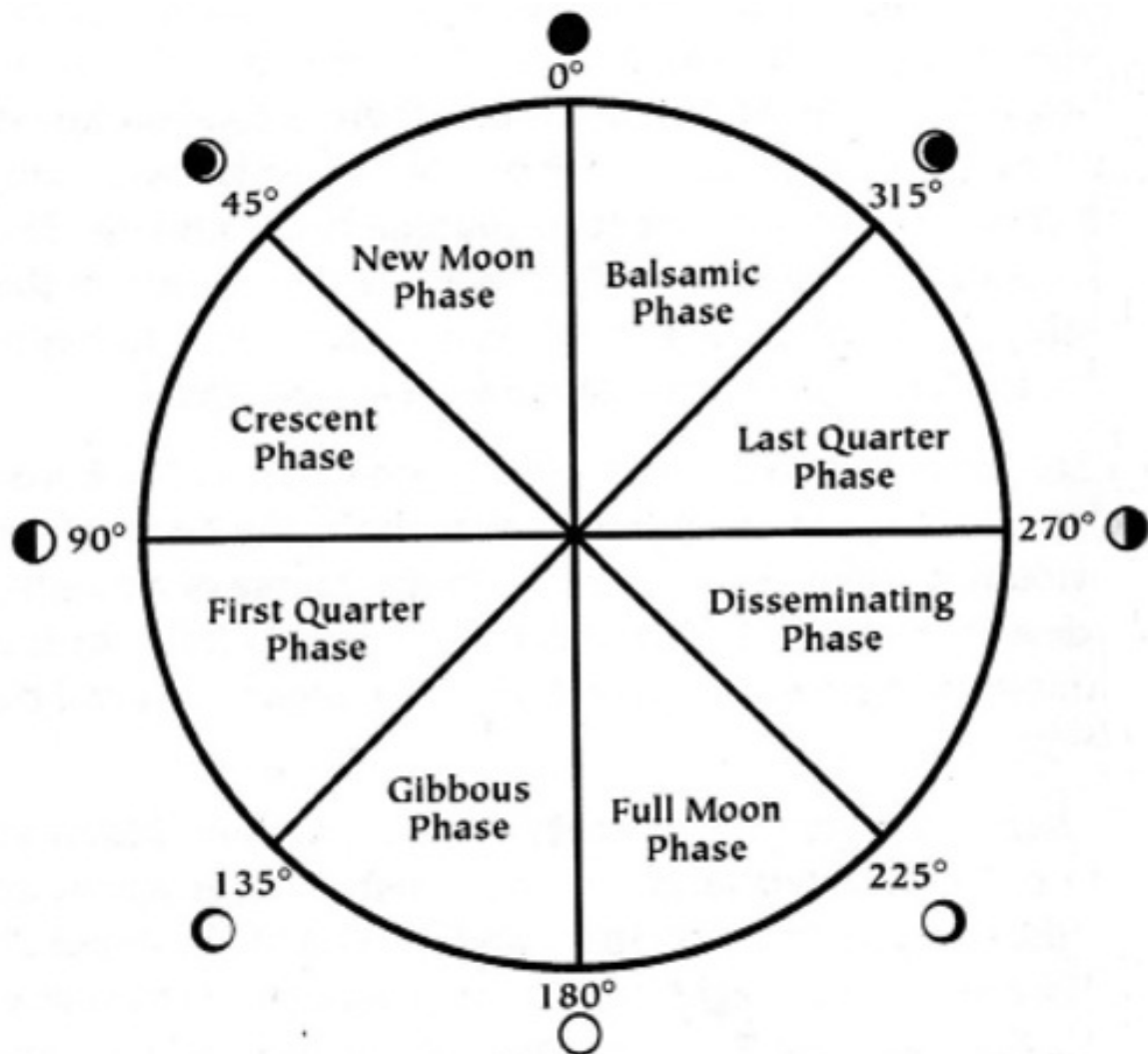
Figure 2-1 Lunar Phases
