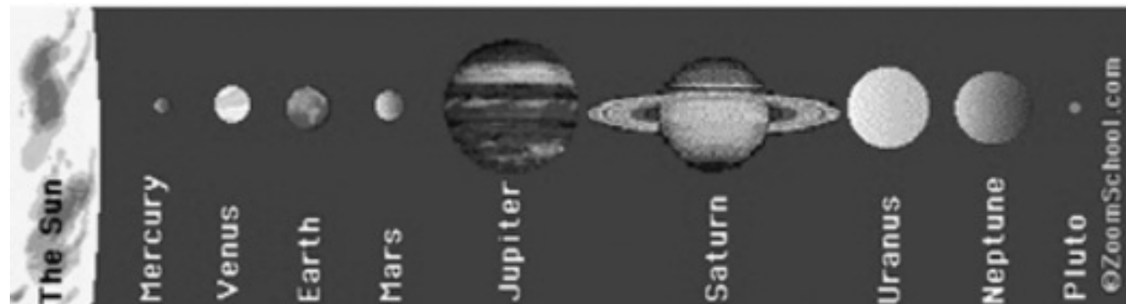
Figure 3-1 The Planets
