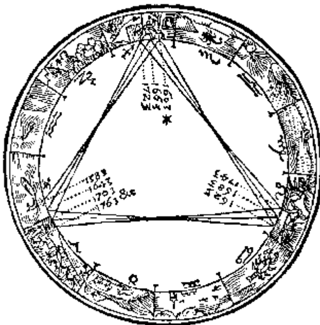
Cycle development of Jupiter and Saturn
