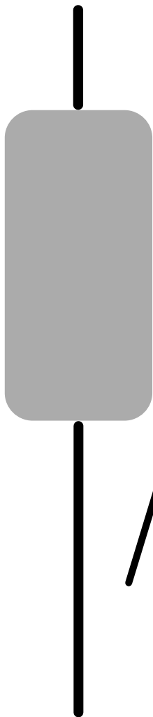
Bearish candle
